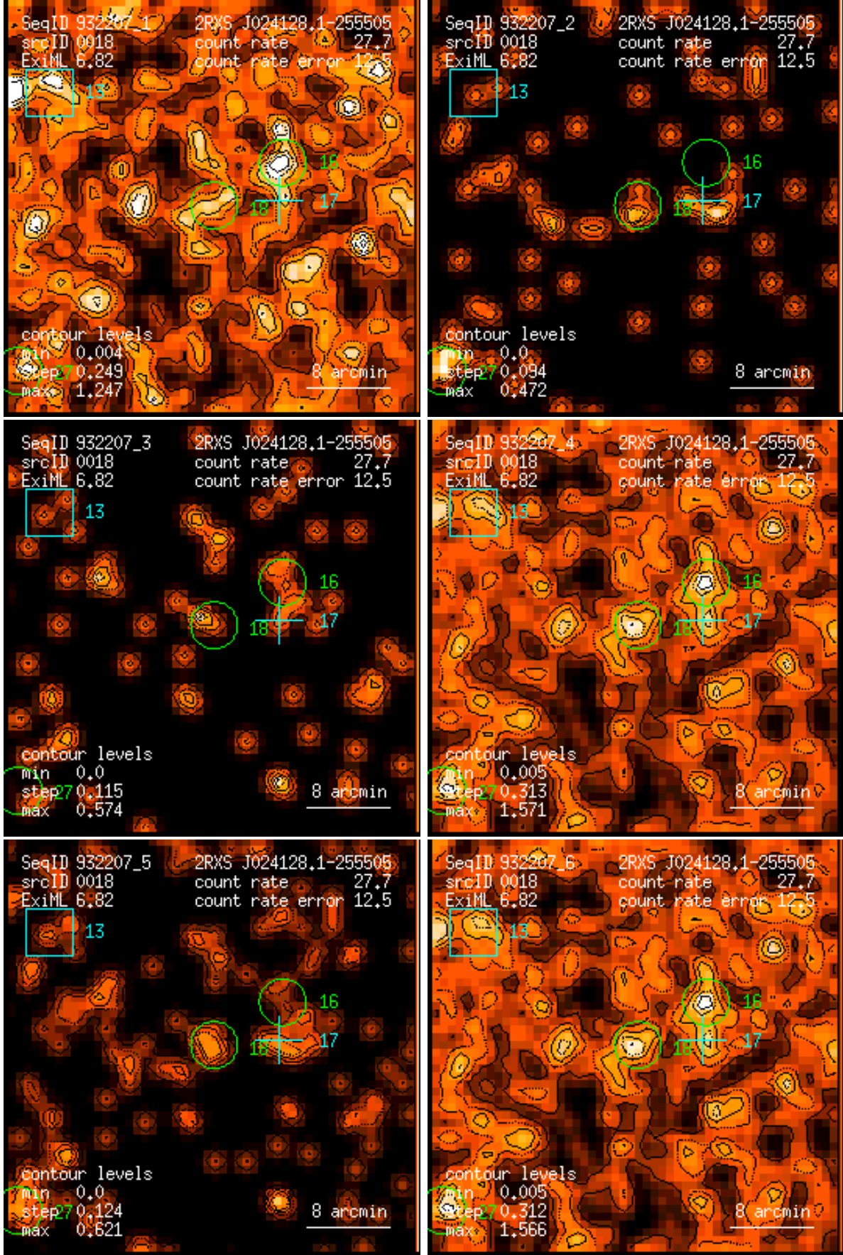
Figure 18: RASS 932207: detection 0018: band rate images, Gaussian filter: (1) PSPC channels 11 – 41, (2) 52 – 90, (3) 91 – 201, (4) 11 – 235, (5) 52 – 201, (6) 11 – 201. Broad band rates in counts/ks. Band rate contour levels in counts/ks/arcmin 2 .
