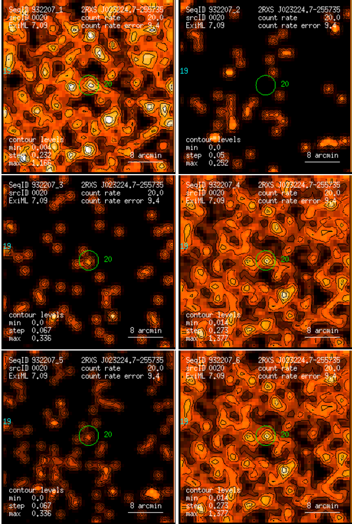
Figure 20: RASS 932207: detection 0020: band rate images, Gaussian filter: (1) PSPC channels 11 – 41, (2) 52 – 90, (3) 91 – 201, (4) 11 – 235, (5) 52 – 201, (6) 11 – 201. Broad band rates in counts/ks. Band rate contour levels in counts/ks/arcmin 2 .
