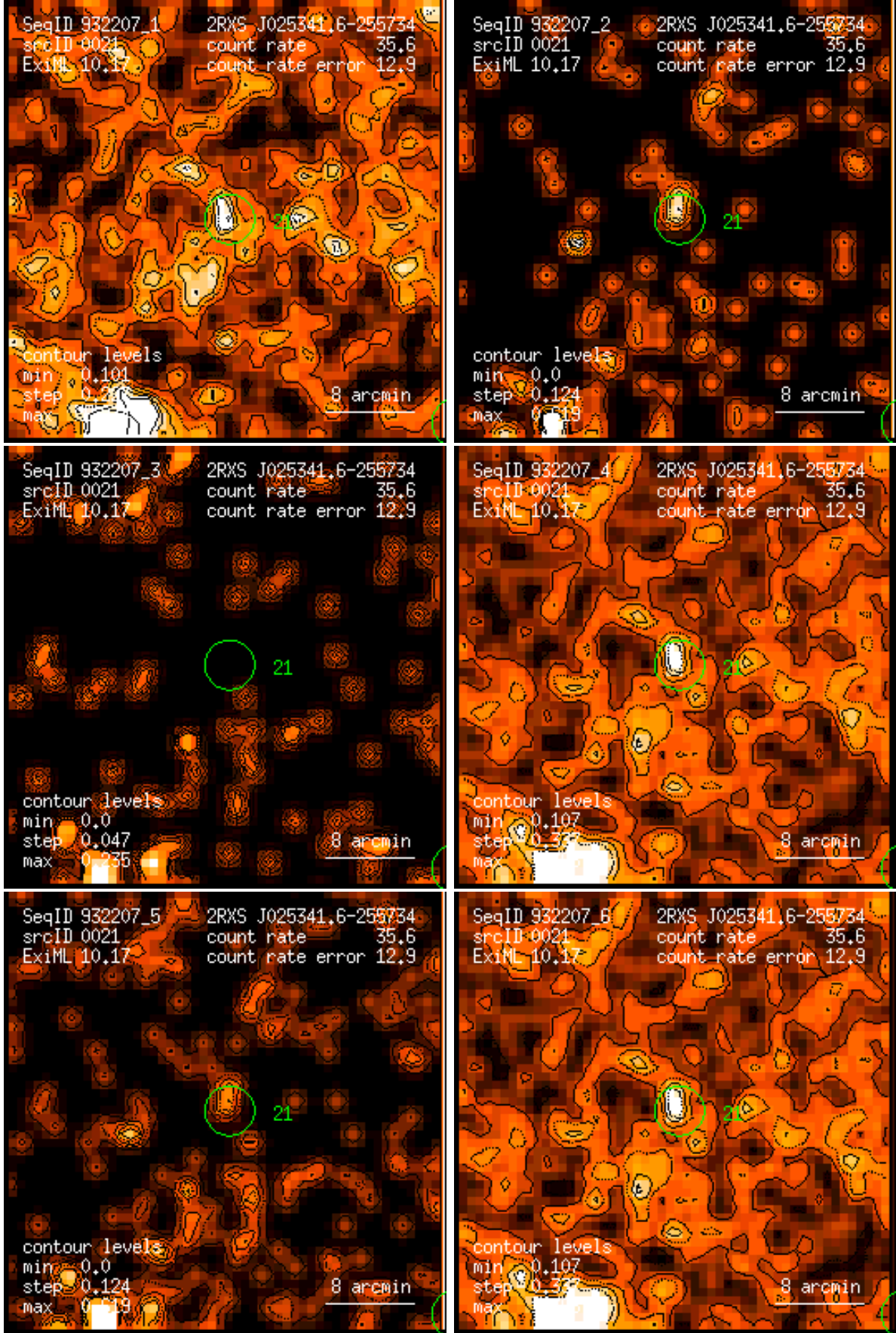
Figure 21: RASS 932207: detection 0021: band rate images, Gaussian filter: (1) PSPC channels 11 – 41, (2) 52 – 90, (3) 91 – 201, (4) 11 – 235, (5) 52 – 201, (6) 11 – 201. Broad band rates in counts/ks. Band rate contour levels in counts/ks/arcmin 2 .
