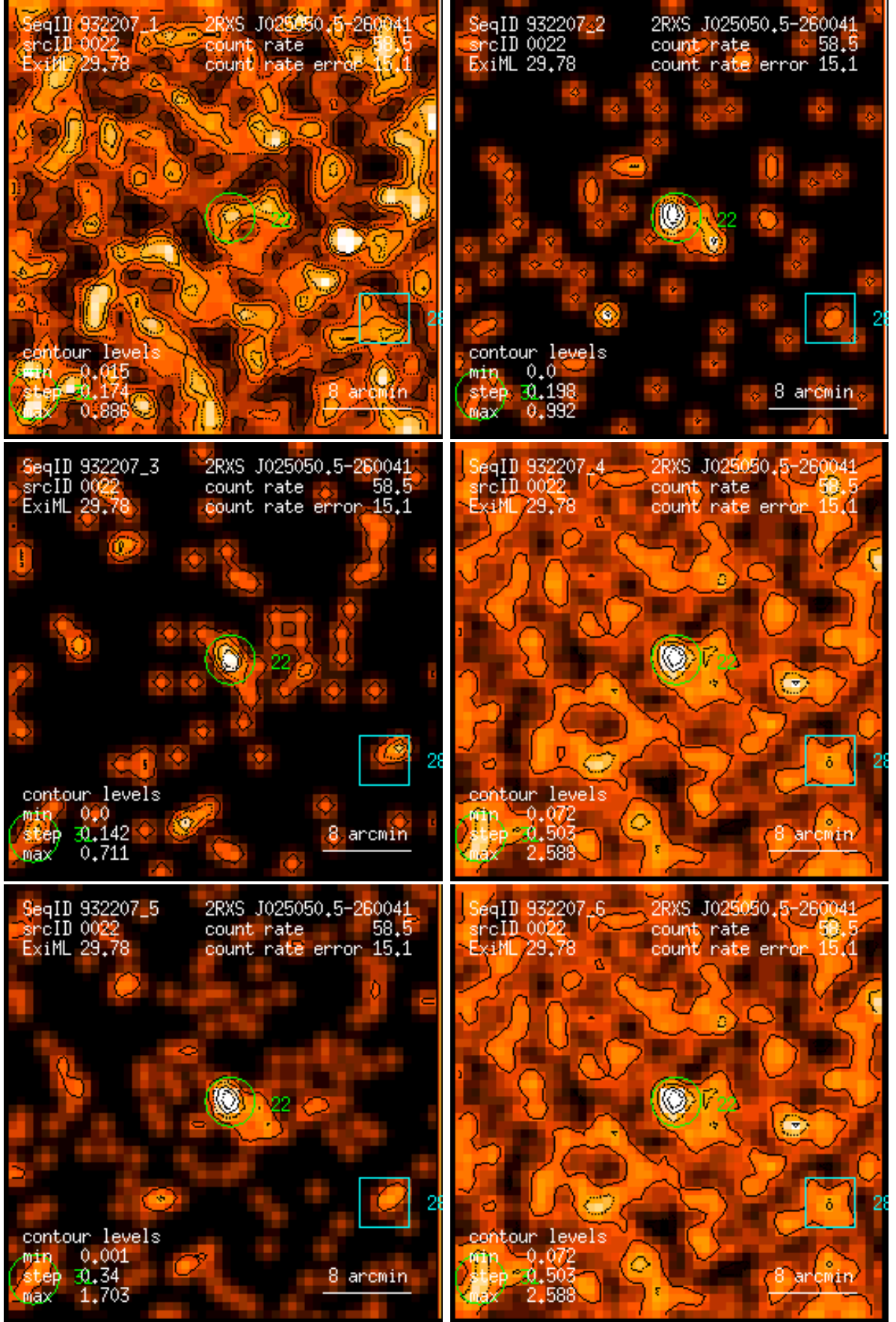
Figure 22: RASS 932207: detection 0022: band rate images, Gaussian filter: (1) PSPC channels 11 – 41, (2) 52 – 90, (3) 91 – 201, (4) 11 – 235, (5) 52 – 201, (6) 11 – 201. Broad band rates in counts/ks. Band rate contour levels in counts/ks/arcmin 2 .
