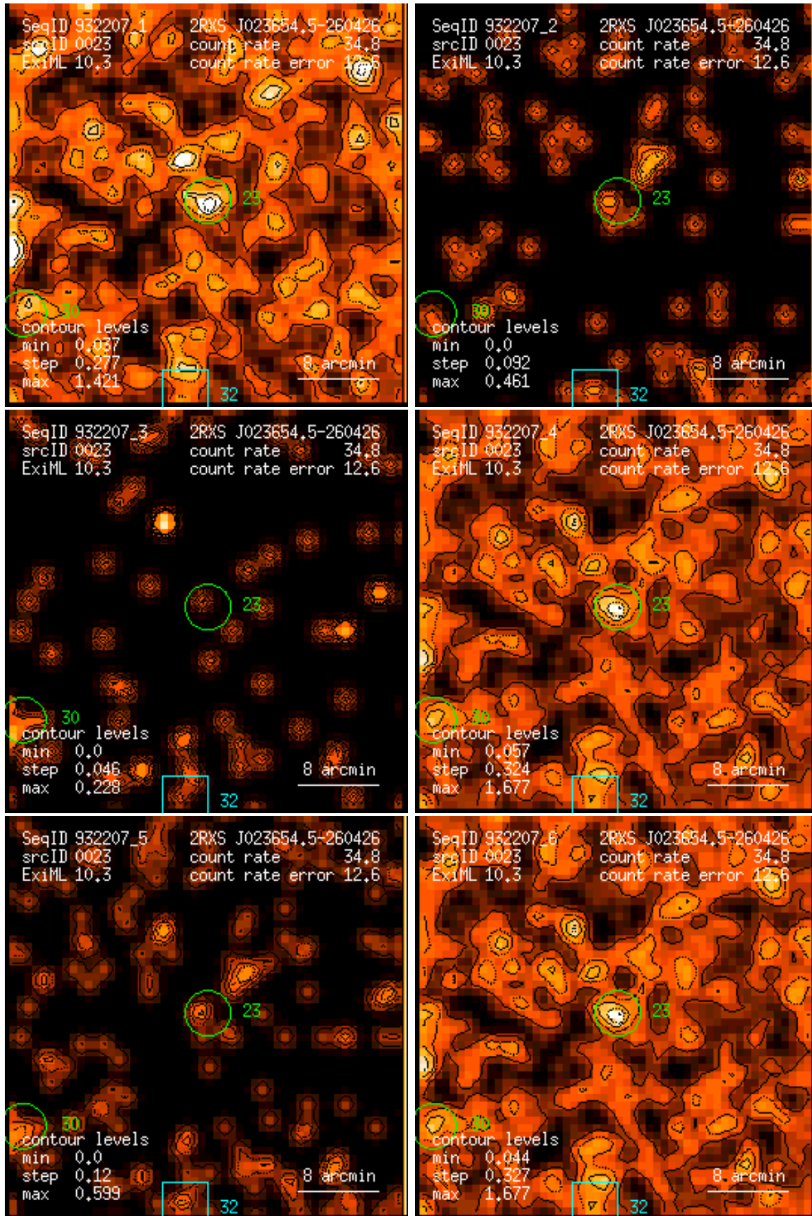
Figure 23: RASS 932207: detection 0023: band rate images, Gaussian filter: (1) PSPC channels 11 – 41, (2) 52 – 90, (3) 91 – 201, (4) 11 – 235, (5) 52 – 201, (6) 11 – 201. Broad band rates in counts/ks. Band rate contour levels in counts/ks/arcmin 2 .
