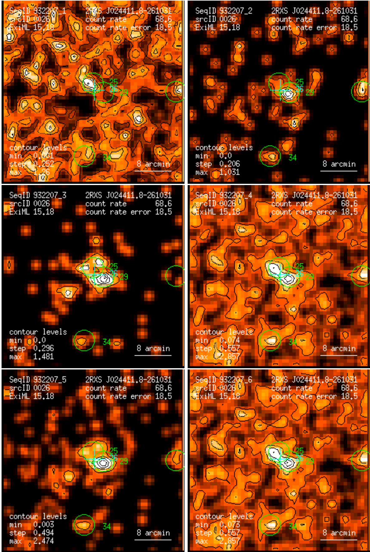
Figure 26: RASS 932207: detection 0026: band rate images, Gaussian filter: (1) PSPC channels 11 – 41, (2) 52 – 90, (3) 91 – 201, (4) 11 – 235, (5) 52 – 201, (6) 11 – 201. Broad band rates in counts/ks. Band rate contour levels in counts/ks/arcmin 2 .
