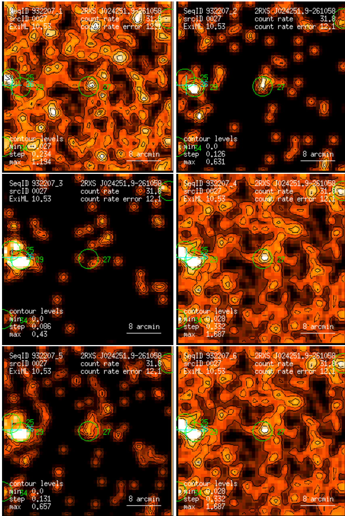
Figure 27: RASS 932207: detection 0027: band rate images, Gaussian filter: (1) PSPC channels 11 – 41, (2) 52 – 90, (3) 91 – 201, (4) 11 – 235, (5) 52 – 201, (6) 11 – 201. Broad band rates in counts/ks. Band rate contour levels in counts/ks/arcmin 2 .
