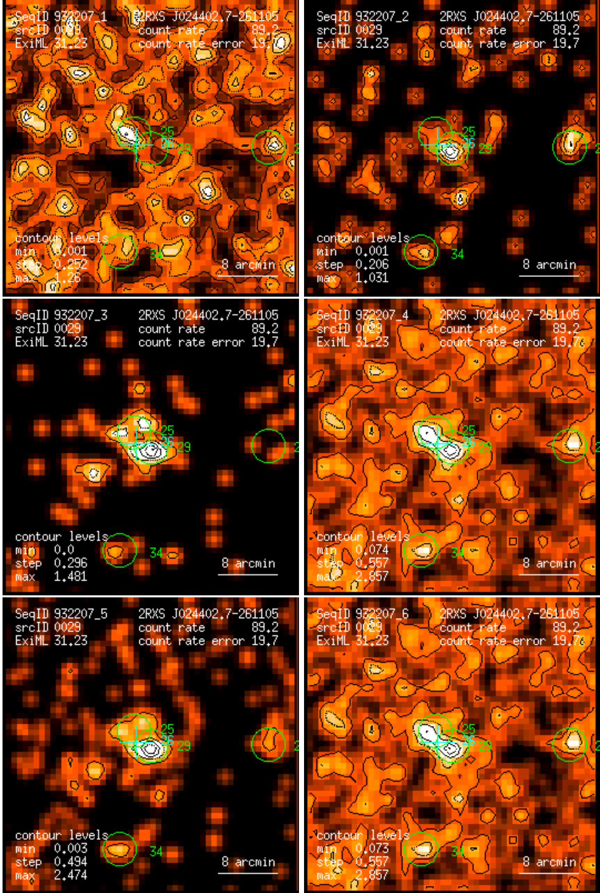
Figure 29: RASS 932207: detection 0029: band rate images, Gaussian filter: (1) PSPC channels 11 – 41, (2) 52 – 90, (3) 91 – 201, (4) 11 – 235, (5) 52 – 201, (6) 11 – 201. Broad band rates in counts/ks. Band rate contour levels in counts/ks/arcmin 2 .
