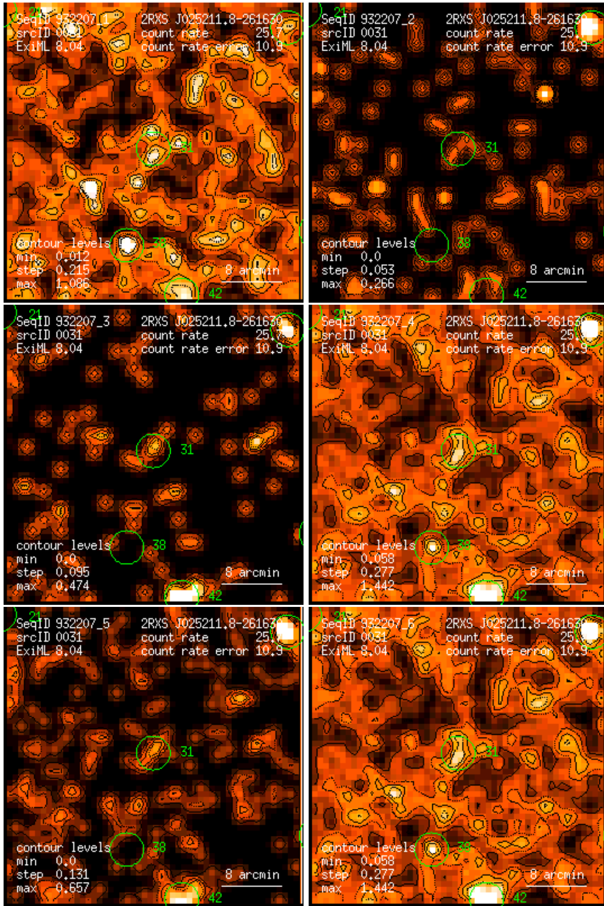
Figure 31: RASS 932207: detection 0031: band rate images, Gaussian filter: (1) PSPC channels 11 – 41, (2) 52 – 90, (3) 91 – 201, (4) 11 – 235, (5) 52 – 201, (6) 11 – 201. Broad band rates in counts/ks. Band rate contour levels in counts/ks/arcmin 2 .
