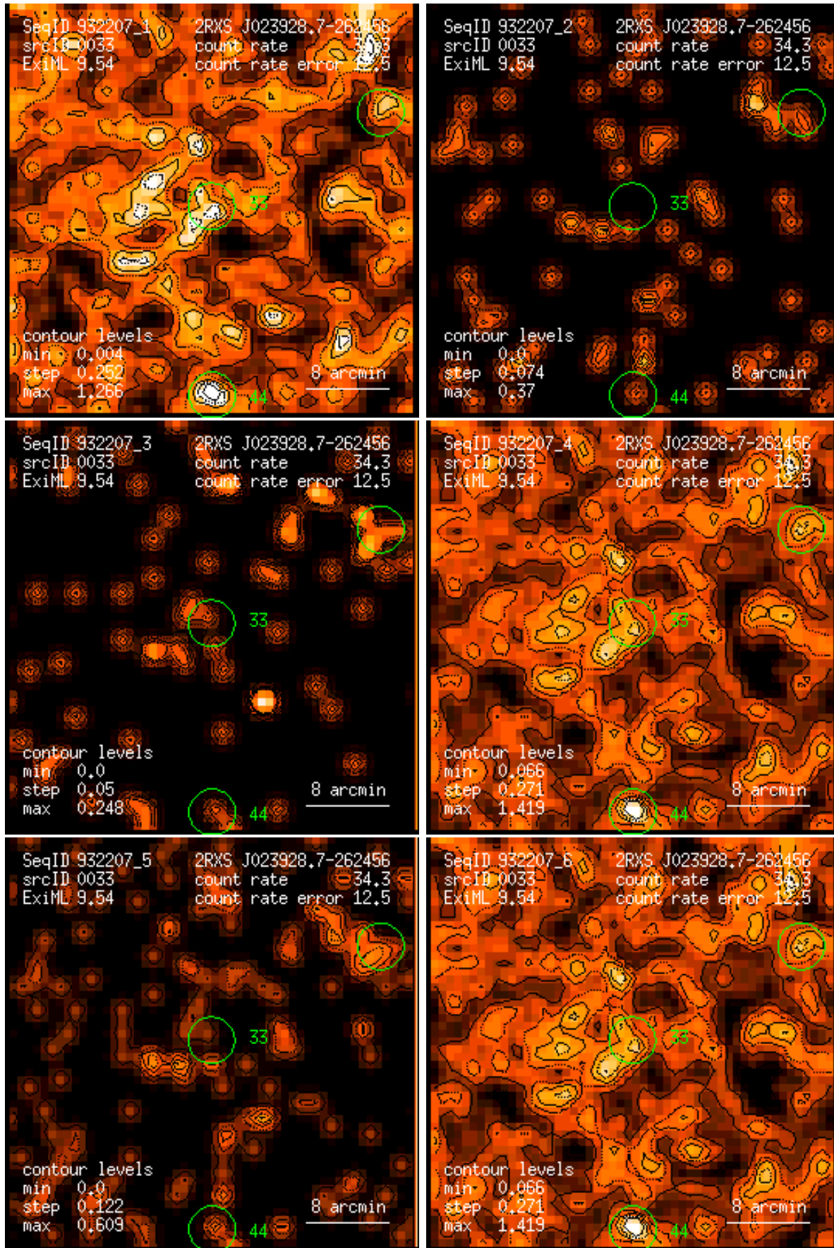
Figure 33: RASS 932207: detection 0033: band rate images, Gaussian filter: (1) PSPC channels 11 – 41, (2) 52 – 90, (3) 91 – 201, (4) 11 – 235, (5) 52 – 201, (6) 11 – 201. Broad band rates in counts/ks. Band rate contour levels in counts/ks/arcmin 2 .
