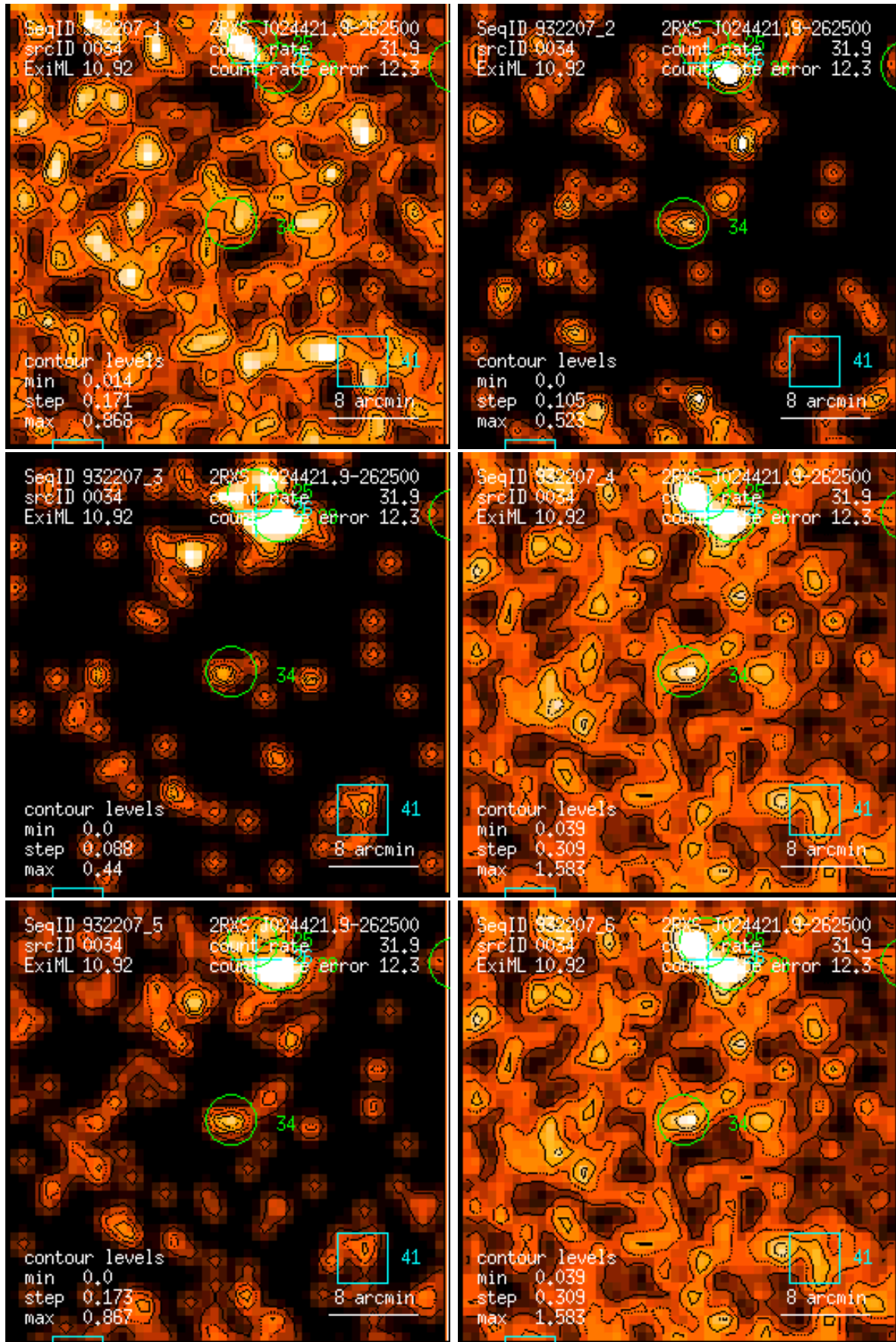
Figure 34: RASS 932207: detection 0034: band rate images, Gaussian filter: (1) PSPC channels 11 – 41, (2) 52 – 90, (3) 91 – 201, (4) 11 – 235, (5) 52 – 201, (6) 11 – 201. Broad band rates in counts/ks. Band rate contour levels in counts/ks/arcmin 2 .
