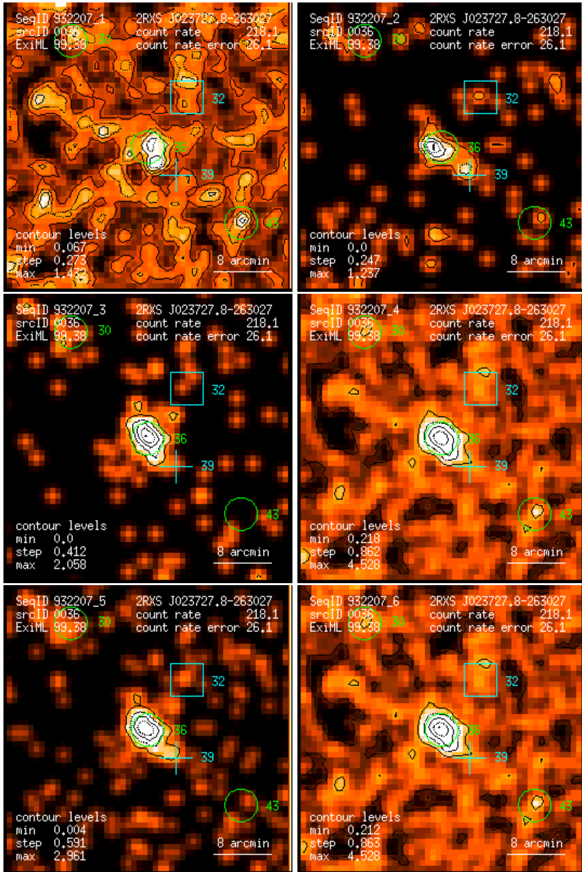
Figure 36: RASS 932207: detection 0036: band rate images, Gaussian filter: (1) PSPC channels 11 – 41, (2) 52 – 90, (3) 91 – 201, (4) 11 – 235, (5) 52 – 201, (6) 11 – 201. Broad band rates in counts/ks. Band rate contour levels in counts/ks/arcmin 2 .
