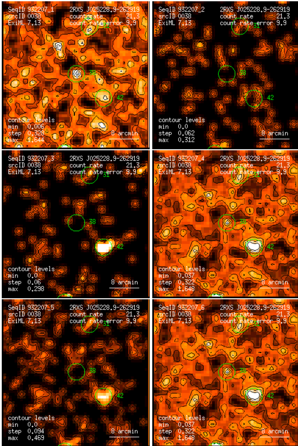
Figure 38: RASS 932207: detection 0038: band rate images, Gaussian filter: (1) PSPC channels 11 – 41, (2) 52 – 90, (3) 91 – 201, (4) 11 – 235, (5) 52 – 201, (6) 11 – 201. Broad band rates in counts/ks. Band rate contour levels in counts/ks/arcmin 2 .
