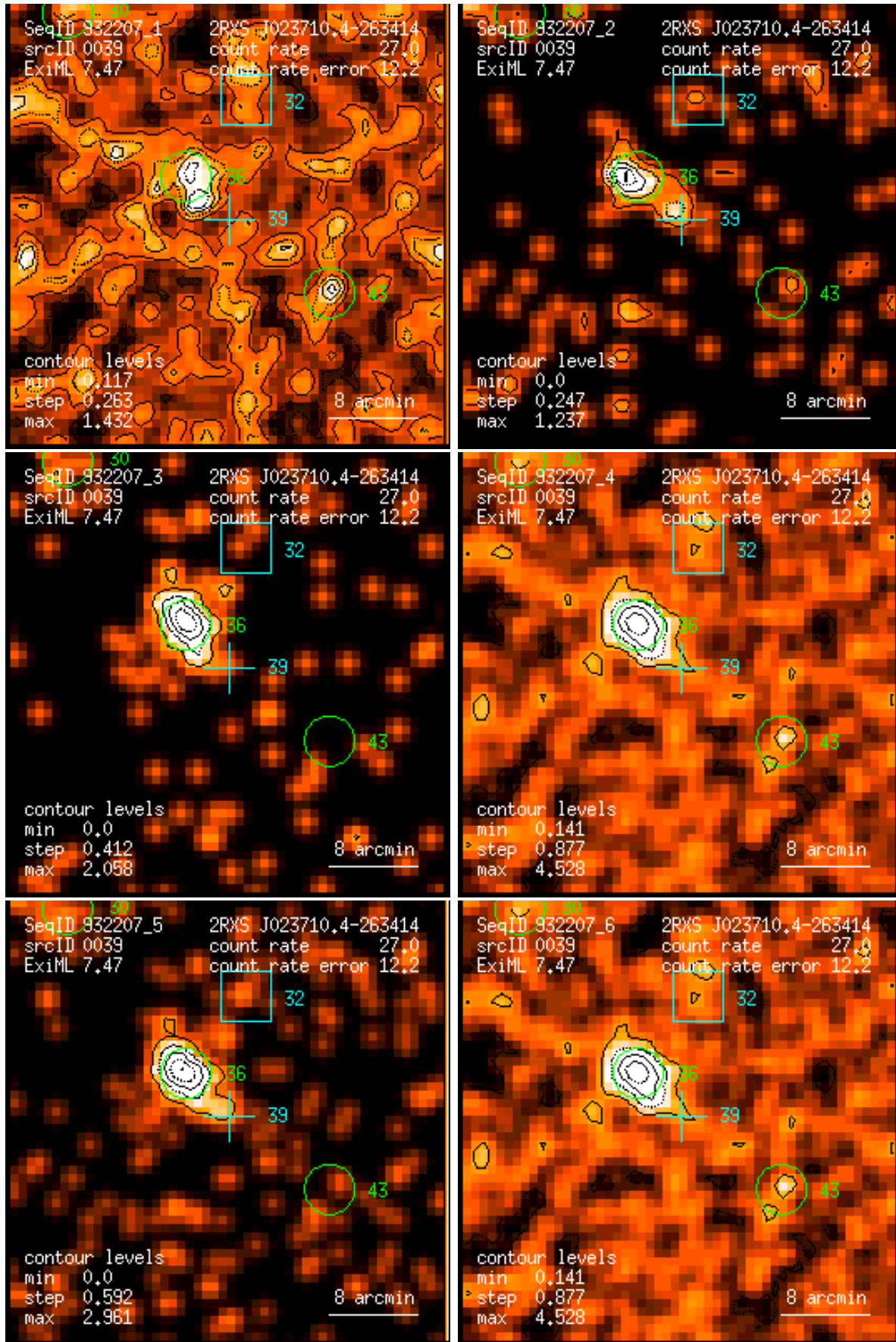
Figure 39: RASS 932207: detection 0039: band rate images, Gaussian filter: (1) PSPC channels 11 – 41, (2) 52 – 90, (3) 91 – 201, (4) 11 – 235, (5) 52 – 201, (6) 11 – 201. Broad band rates in counts/ks. Band rate contour levels in counts/ks/arcmin 2 .
