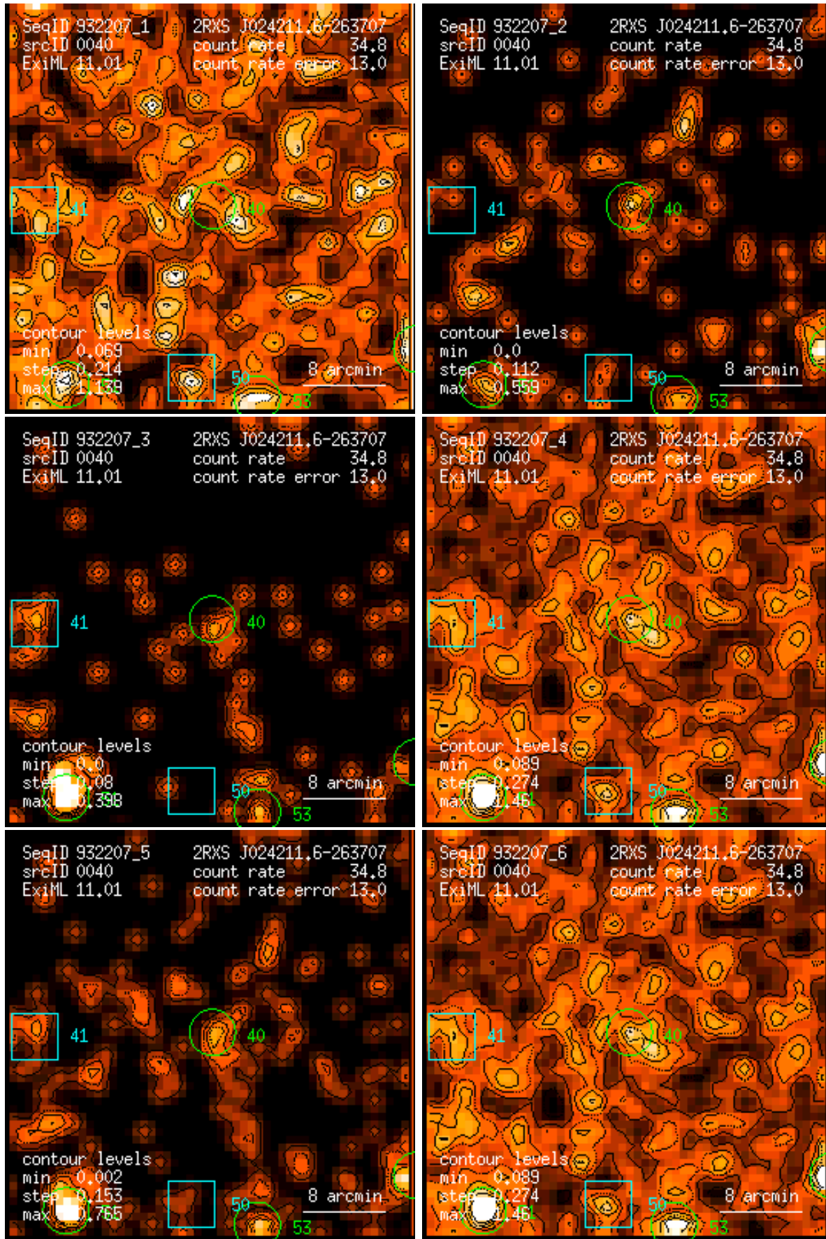
Figure 40: RASS 932207: detection 0040: band rate images, Gaussian filter: (1) PSPC channels 11 – 41, (2) 52 – 90, (3) 91 – 201, (4) 11 – 235, (5) 52 – 201, (6) 11 – 201. Broad band rates in counts/ks. Band rate contour levels in counts/ks/arcmin 2 .
