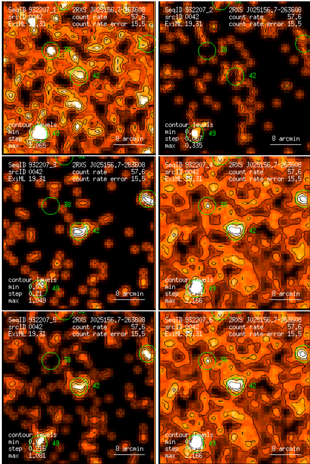
Figure 42: RASS 932207: detection 0042: band rate images, Gaussian filter: (1) PSPC channels 11 – 41, (2) 52 – 90, (3) 91 – 201, (4) 11 – 235, (5) 52 – 201, (6) 11 – 201. Broad band rates in counts/ks. Band rate contour levels in counts/ks/arcmin 2 .
