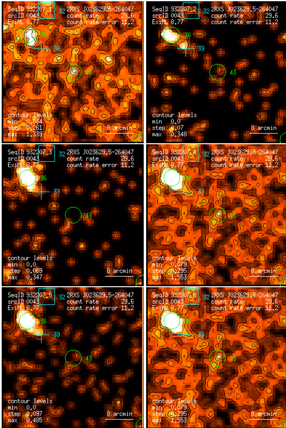
Figure 43: RASS 932207: detection 0043: band rate images, Gaussian filter: (1) PSPC channels 11 – 41, (2) 52 – 90, (3) 91 – 201, (4) 11 – 235, (5) 52 – 201, (6) 11 – 201. Broad band rates in counts/ks. Band rate contour levels in counts/ks/arcmin 2 .
