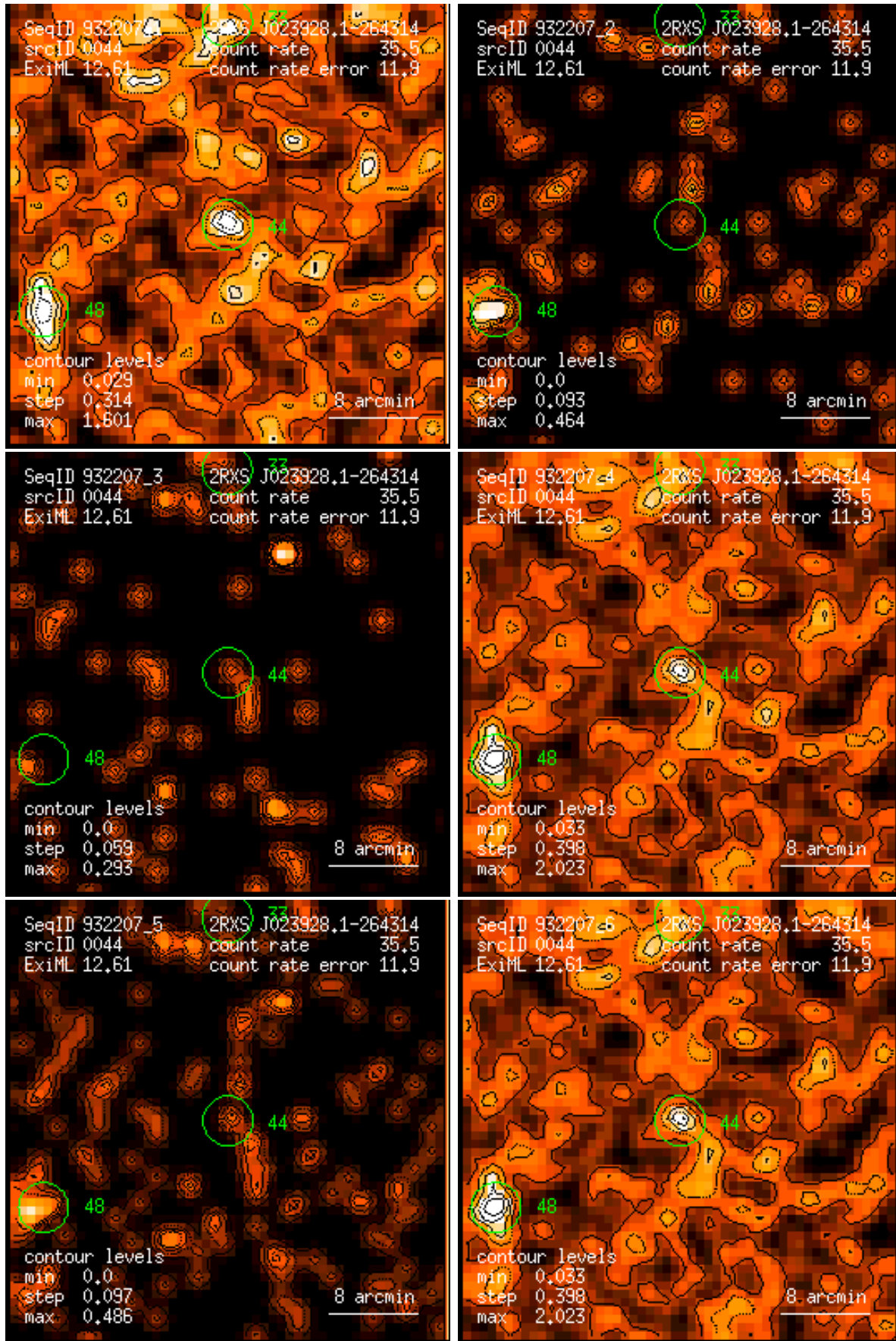
Figure 44: RASS 932207: detection 0044: band rate images, Gaussian filter: (1) PSPC channels 11 – 41, (2) 52 – 90, (3) 91 – 201, (4) 11 – 235, (5) 52 – 201, (6) 11 – 201. Broad band rates in counts/ks. Band rate contour levels in counts/ks/arcmin 2 .
