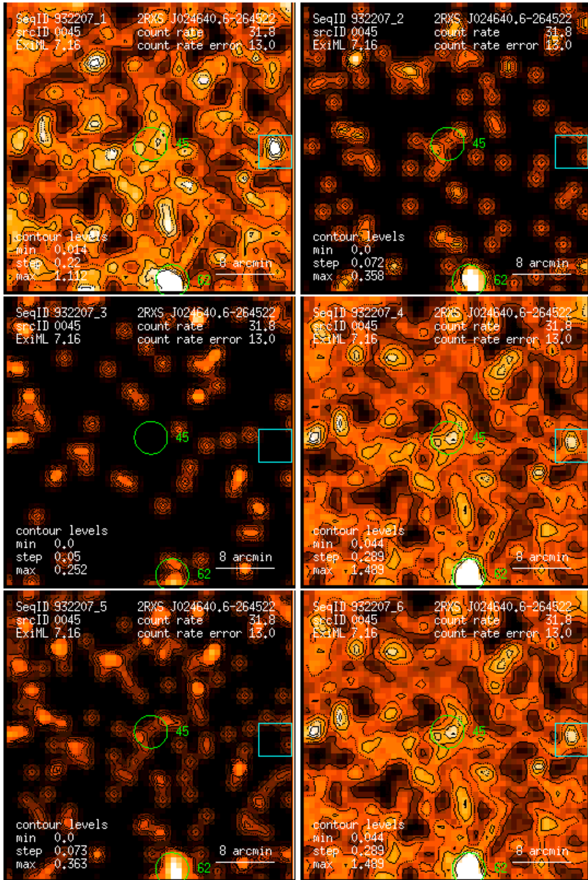
Figure 45: RASS 932207: detection 0045: band rate images, Gaussian filter: (1) PSPC channels 11 – 41, (2) 52 – 90, (3) 91 – 201, (4) 11 – 235, (5) 52 – 201, (6) 11 – 201. Broad band rates in counts/ks. Band rate contour levels in counts/ks/arcmin 2 .
