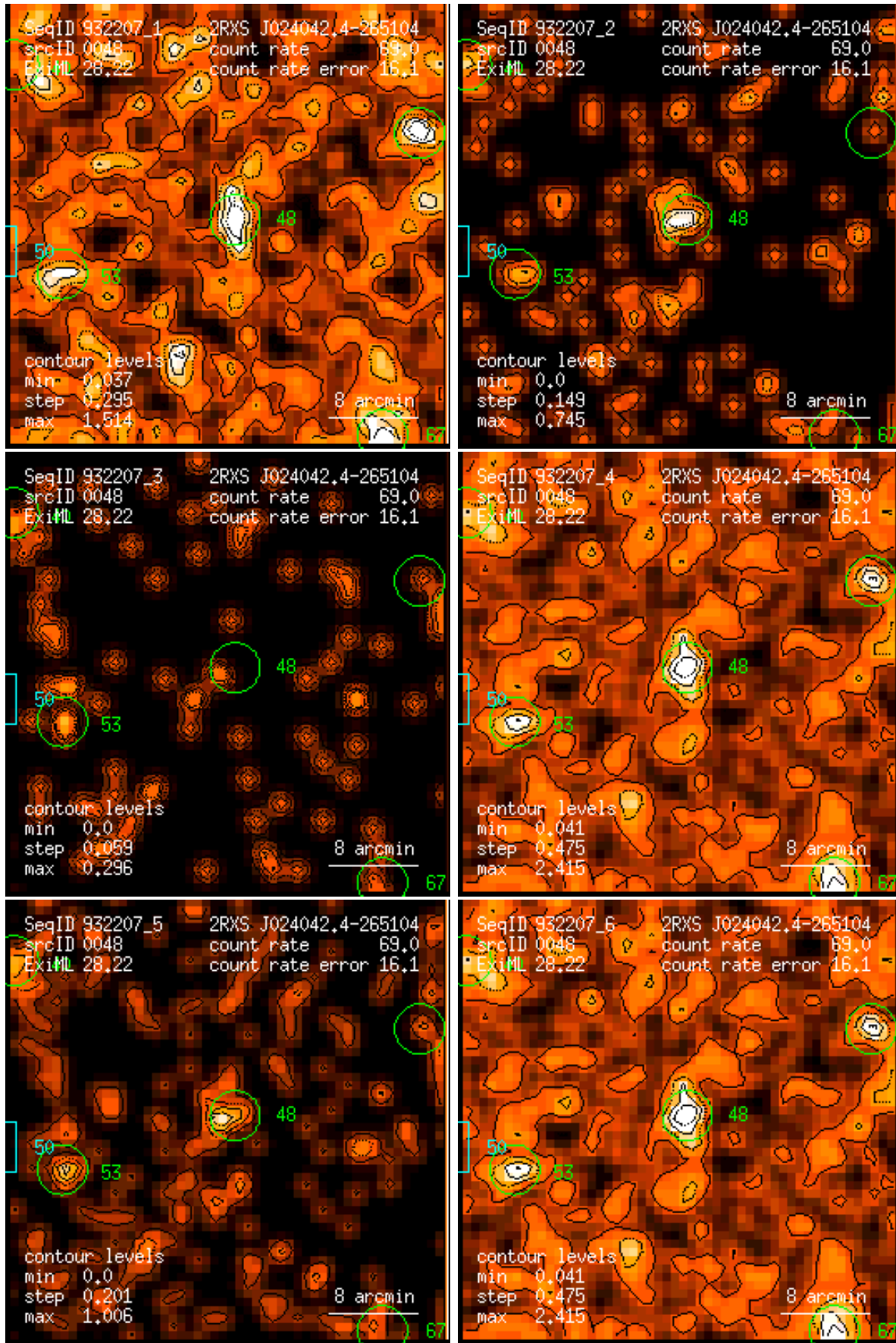
Figure 48: RASS 932207: detection 0048: band rate images, Gaussian filter: (1) PSPC channels 11 – 41, (2) 52 – 90, (3) 91 – 201, (4) 11 – 235, (5) 52 – 201, (6) 11 – 201. Broad band rates in counts/ks. Band rate contour levels in counts/ks/arcmin 2 .
