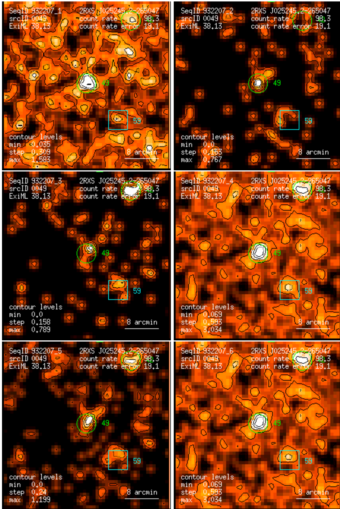
Figure 49: RASS 932207: detection 0049: band rate images, Gaussian filter: (1) PSPC channels 11 – 41, (2) 52 – 90, (3) 91 – 201, (4) 11 – 235, (5) 52 – 201, (6) 11 – 201. Broad band rates in counts/ks. Band rate contour levels in counts/ks/arcmin 2 .
