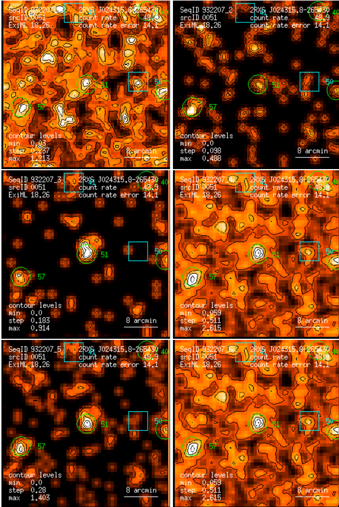
Figure 51: RASS 932207: detection 0051: band rate images, Gaussian filter: (1) PSPC channels 11 – 41, (2) 52 – 90, (3) 91 – 201, (4) 11 – 235, (5) 52 – 201, (6) 11 – 201. Broad band rates in counts/ks. Band rate contour levels in counts/ks/arcmin 2 .
