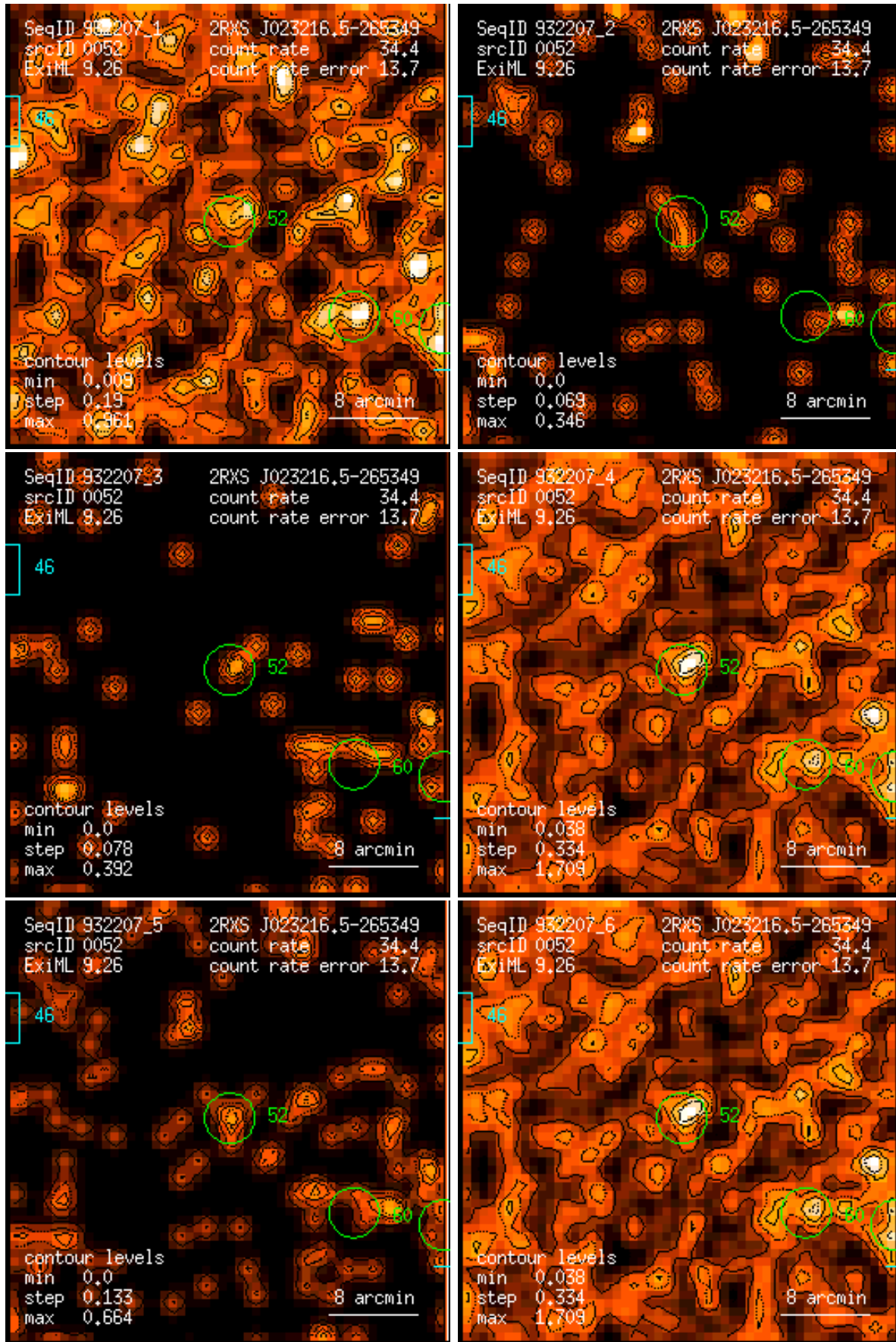
Figure 52: RASS 932207: detection 0052: band rate images, Gaussian filter: (1) PSPC channels 11 – 41, (2) 52 – 90, (3) 91 – 201, (4) 11 – 235, (5) 52 – 201, (6) 11 – 201. Broad band rates in counts/ks. Band rate contour levels in counts/ks/arcmin 2 .
