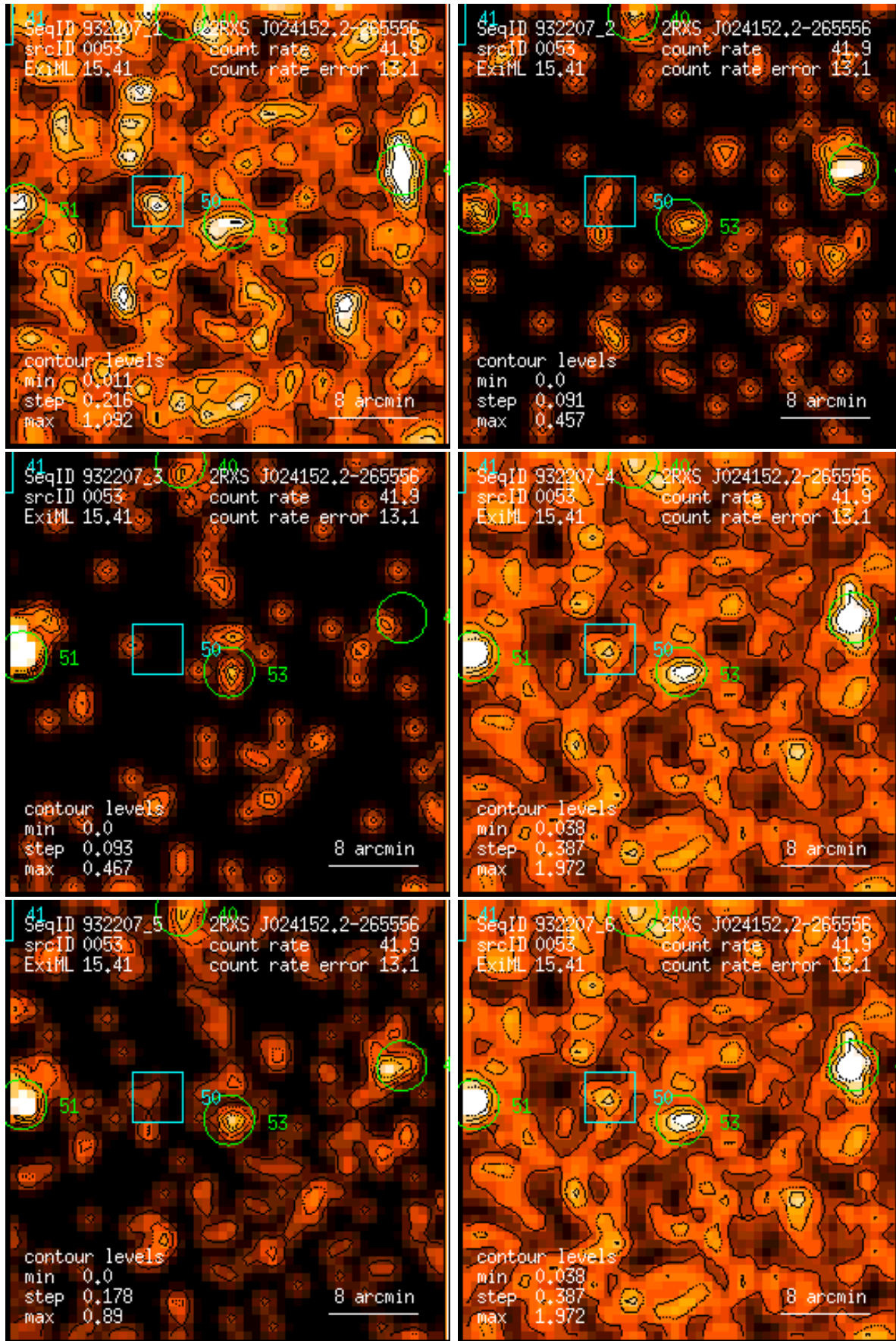
Figure 53: RASS 932207: detection 0053: band rate images, Gaussian filter: (1) PSPC channels 11 – 41, (2) 52 – 90, (3) 91 – 201, (4) 11 – 235, (5) 52 – 201, (6) 11 – 201. Broad band rates in counts/ks. Band rate contour levels in counts/ks/arcmin 2 .
