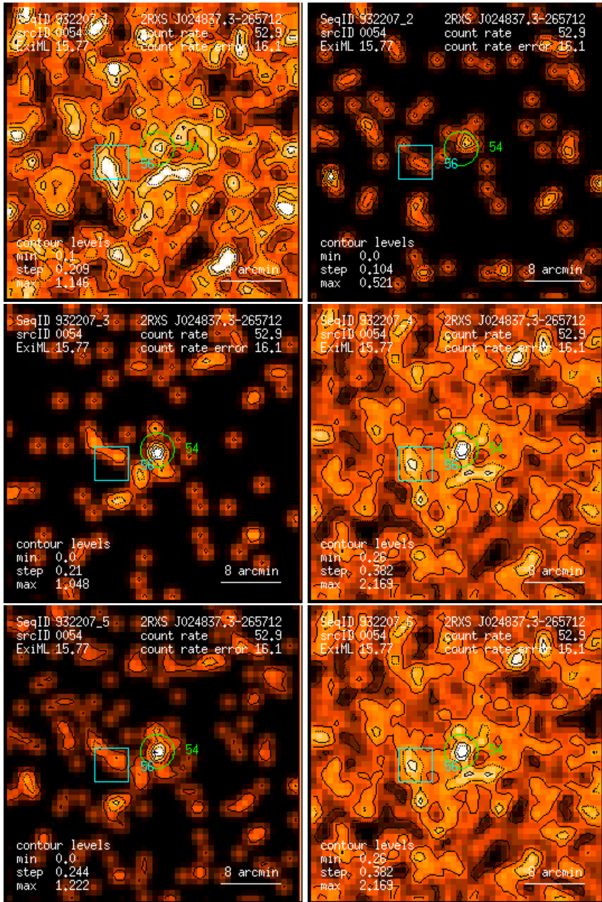
Figure 54: RASS 932207: detection 0054: band rate images, Gaussian filter: (1) PSPC channels 11 – 41, (2) 52 – 90, (3) 91 – 201, (4) 11 – 235, (5) 52 – 201, (6) 11 – 201. Broad band rates in counts/ks. Band rate contour levels in counts/ks/arcmin 2 .
