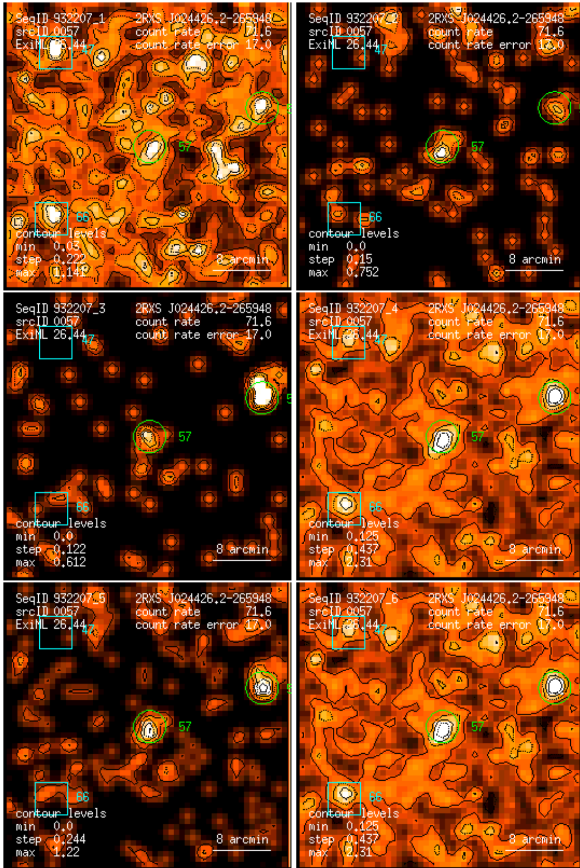
Figure 57: RASS 932207: detection 0057: band rate images, Gaussian filter: (1) PSPC channels 11 – 41, (2) 52 – 90, (3) 91 – 201, (4) 11 – 235, (5) 52 – 201, (6) 11 – 201. Broad band rates in counts/ks. Band rate contour levels in counts/ks/arcmin 2 .
