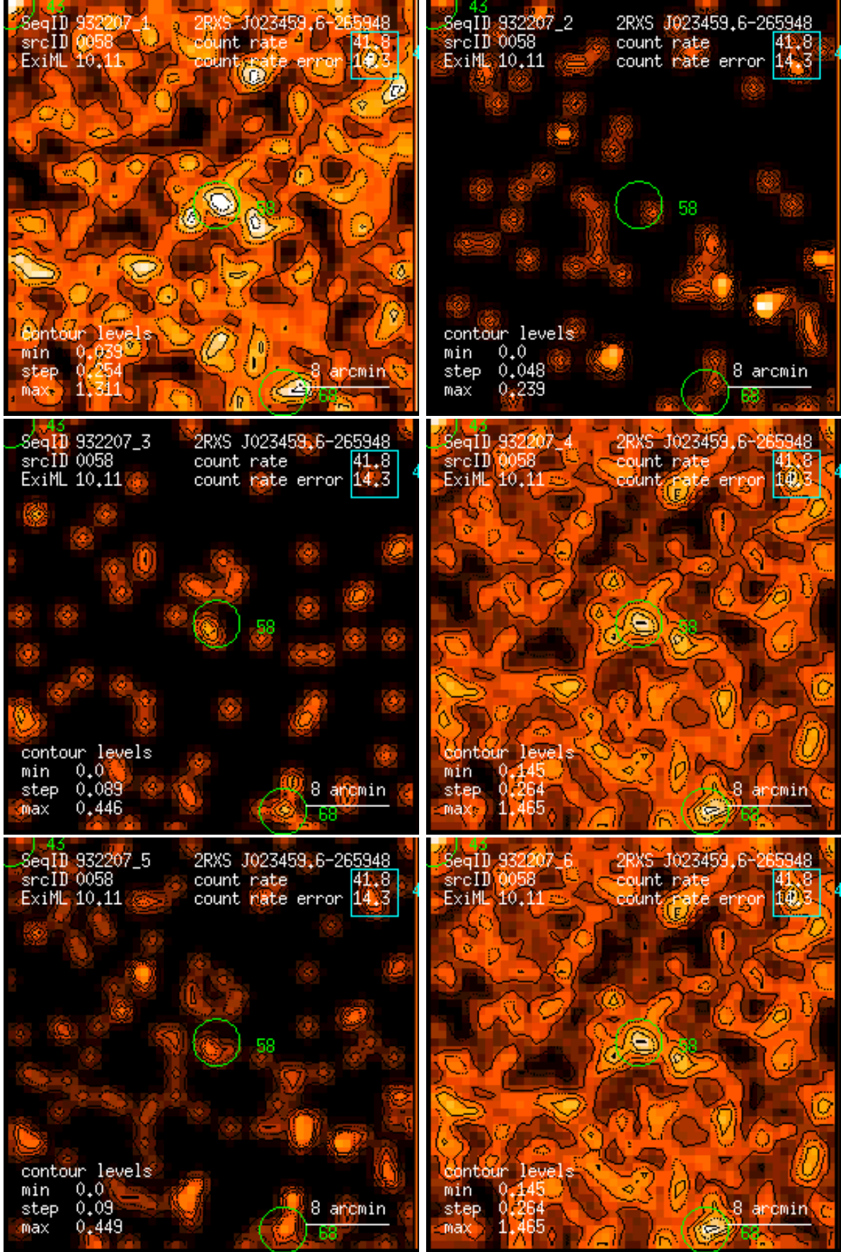
Figure 58: RASS 932207: detection 0058: band rate images, Gaussian filter: (1) PSPC channels 11 – 41, (2) 52 – 90, (3) 91 – 201, (4) 11 – 235, (5) 52 – 201, (6) 11 – 201. Broad band rates in counts/ks. Band rate contour levels in counts/ks/arcmin 2 .
