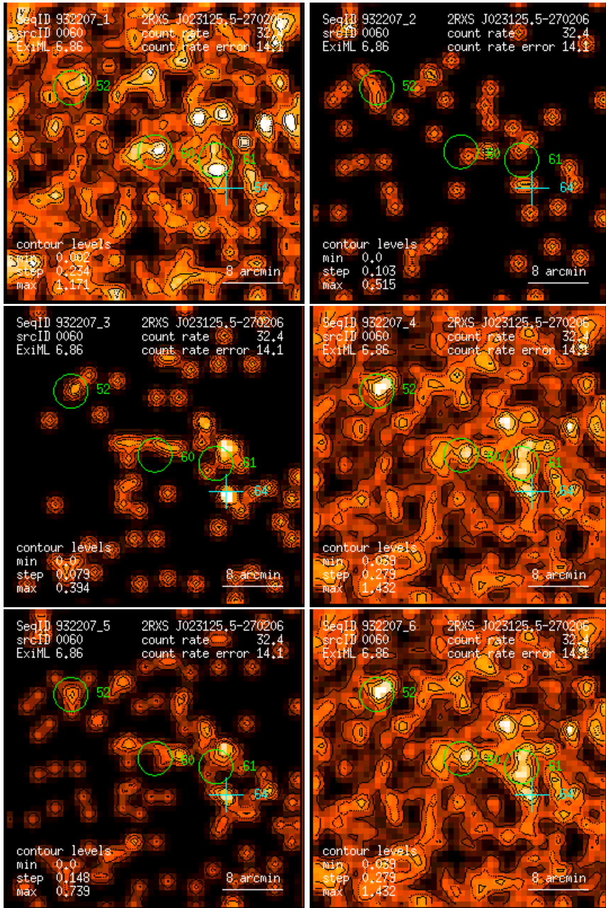
Figure 60: RASS 932207: detection 0060: band rate images, Gaussian filter: (1) PSPC channels 11 – 41, (2) 52 – 90, (3) 91 – 201, (4) 11 – 235, (5) 52 – 201, (6) 11 – 201. Broad band rates in counts/ks. Band rate contour levels in counts/ks/arcmin 2 .
