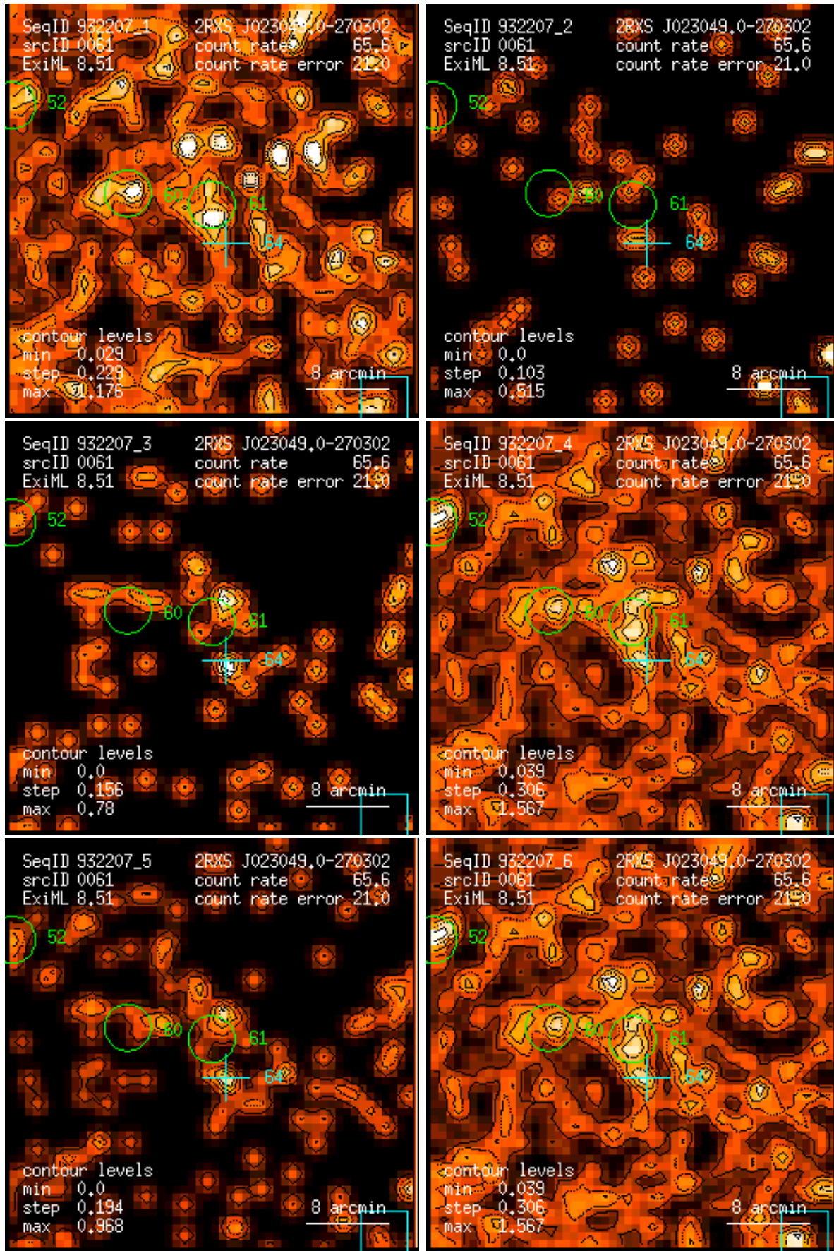
Figure 61: RASS 932207: detection 0061: band rate images, Gaussian filter: (1) PSPC channels 11 – 41, (2) 52 – 90, (3) 91 – 201, (4) 11 – 235, (5) 52 – 201, (6) 11 – 201. Broad band rates in counts/ks. Band rate contour levels in counts/ks/arcmin 2 .
