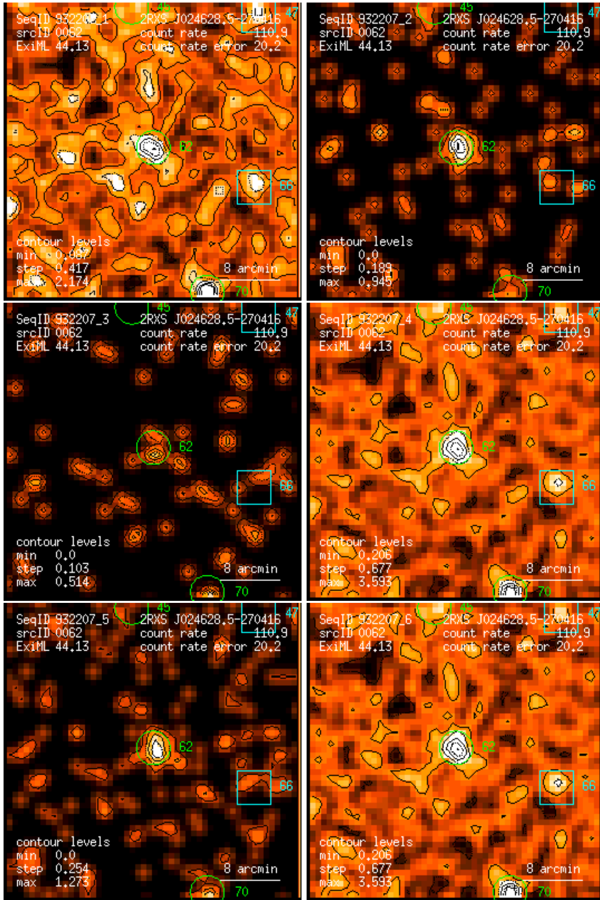
Figure 62: RASS 932207: detection 0062: band rate images, Gaussian filter: (1) PSPC channels 11 – 41, (2) 52 – 90, (3) 91 – 201, (4) 11 – 235, (5) 52 – 201, (6) 11 – 201. Broad band rates in counts/ks. Band rate contour levels in counts/ks/arcmin 2 .
