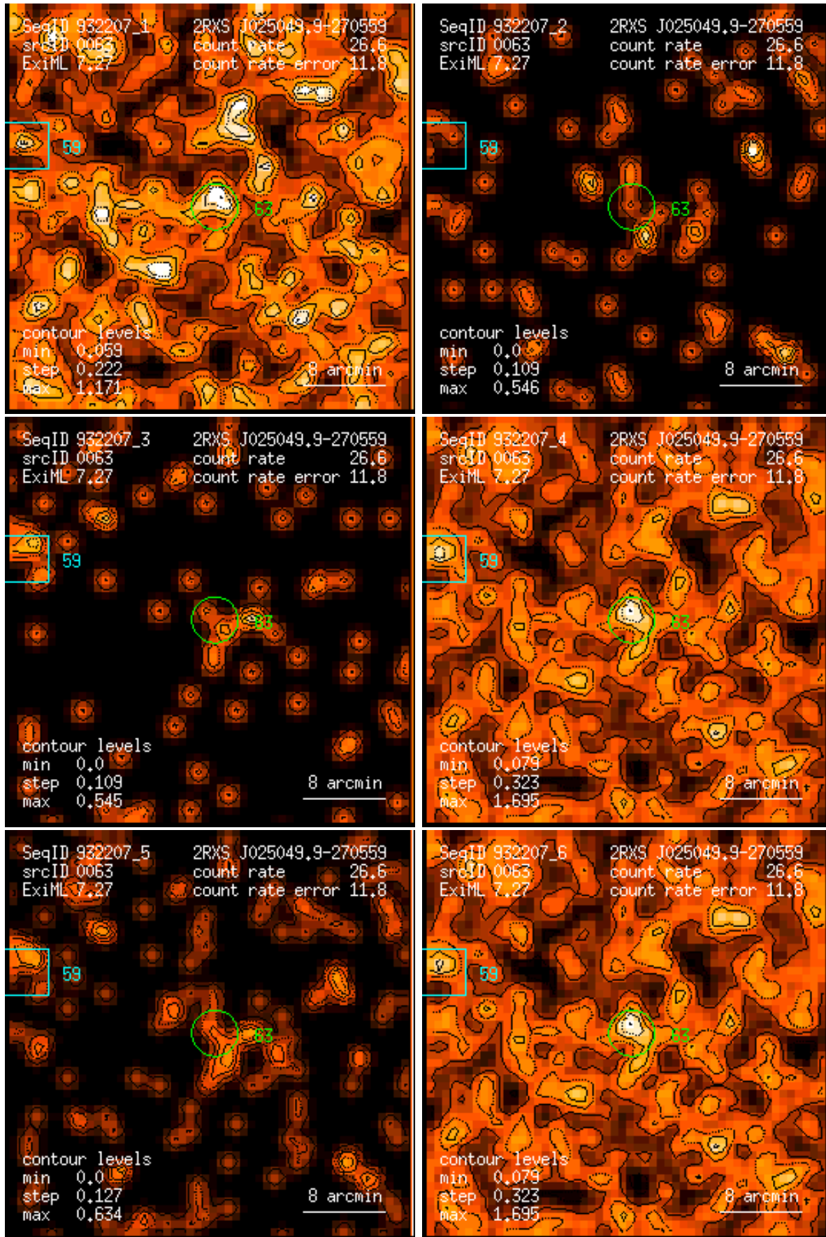
Figure 63: RASS 932207: detection 0063: band rate images, Gaussian filter: (1) PSPC channels 11 – 41, (2) 52 – 90, (3) 91 – 201, (4) 11 – 235, (5) 52 – 201, (6) 11 – 201. Broad band rates in counts/ks. Band rate contour levels in counts/ks/arcmin 2 .
