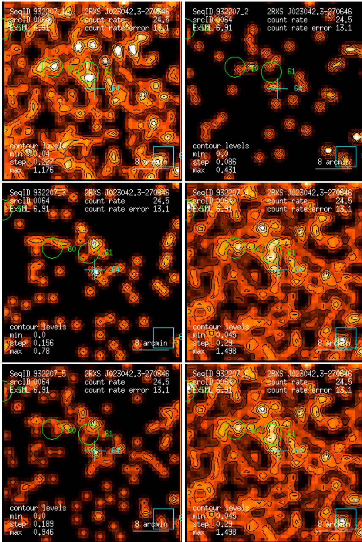
Figure 64: RASS 932207: detection 0064: band rate images, Gaussian filter: (1) PSPC channels 11 – 41, (2) 52 – 90, (3) 91 – 201, (4) 11 – 235, (5) 52 – 201, (6) 11 – 201. Broad band rates in counts/ks. Band rate contour levels in counts/ks/arcmin 2 .
