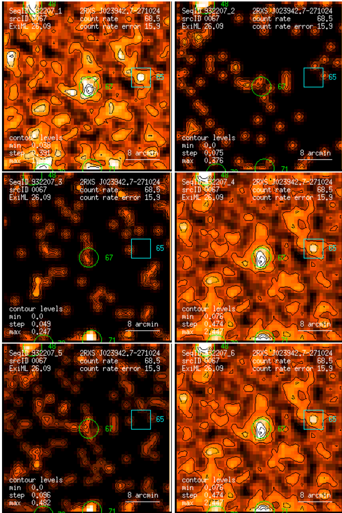
Figure 67: RASS 932207: detection 0067: band rate images, Gaussian filter: (1) PSPC channels 11 – 41, (2) 52 – 90, (3) 91 – 201, (4) 11 – 235, (5) 52 – 201, (6) 11 – 201. Broad band rates in counts/ks. Band rate contour levels in counts/ks/arcmin 2 .
