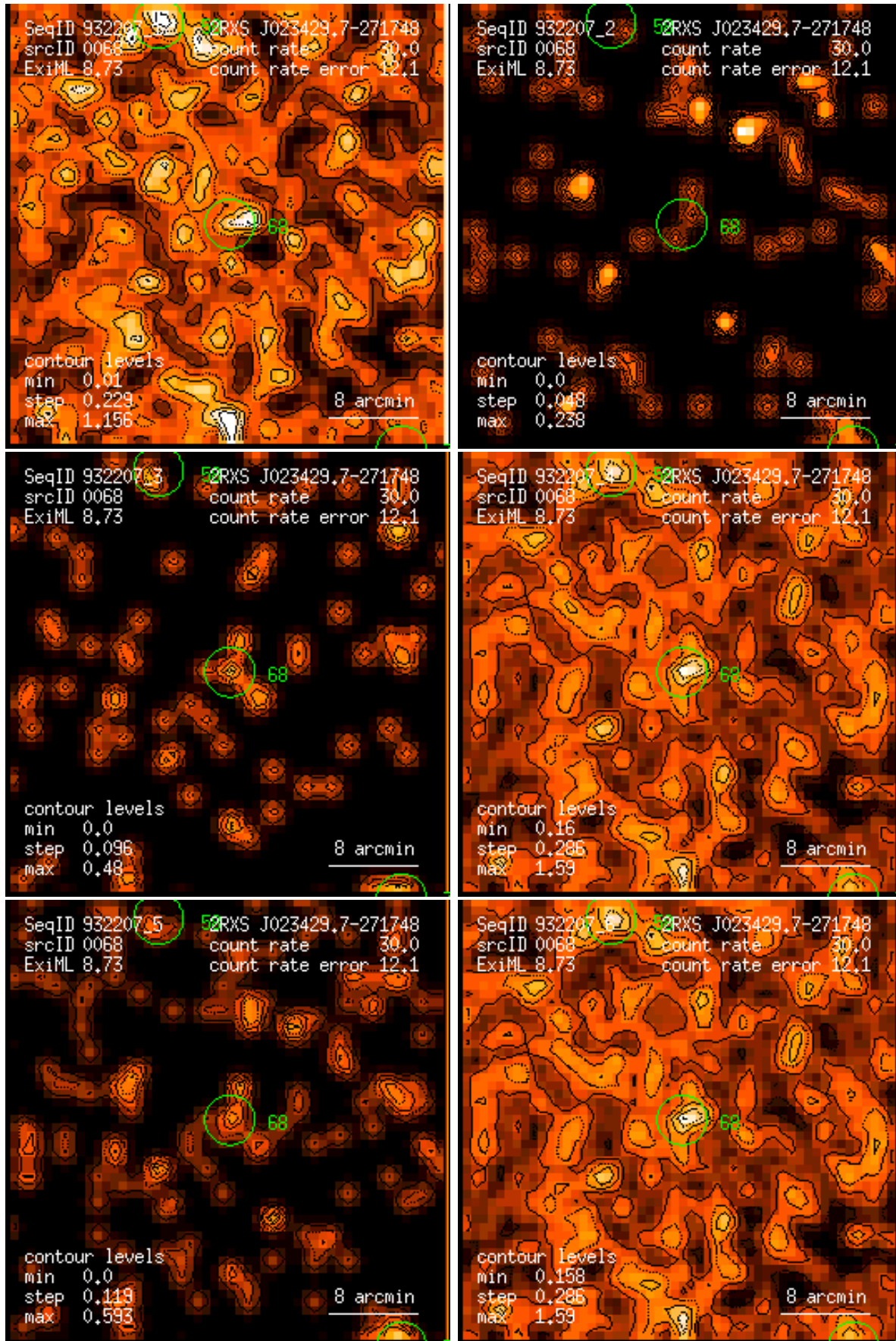
Figure 68: RASS 932207: detection 0068: band rate images, Gaussian filter: (1) PSPC channels 11 – 41, (2) 52 – 90, (3) 91 – 201, (4) 11 – 235, (5) 52 – 201, (6) 11 – 201. Broad band rates in counts/ks. Band rate contour levels in counts/ks/arcmin 2 .
