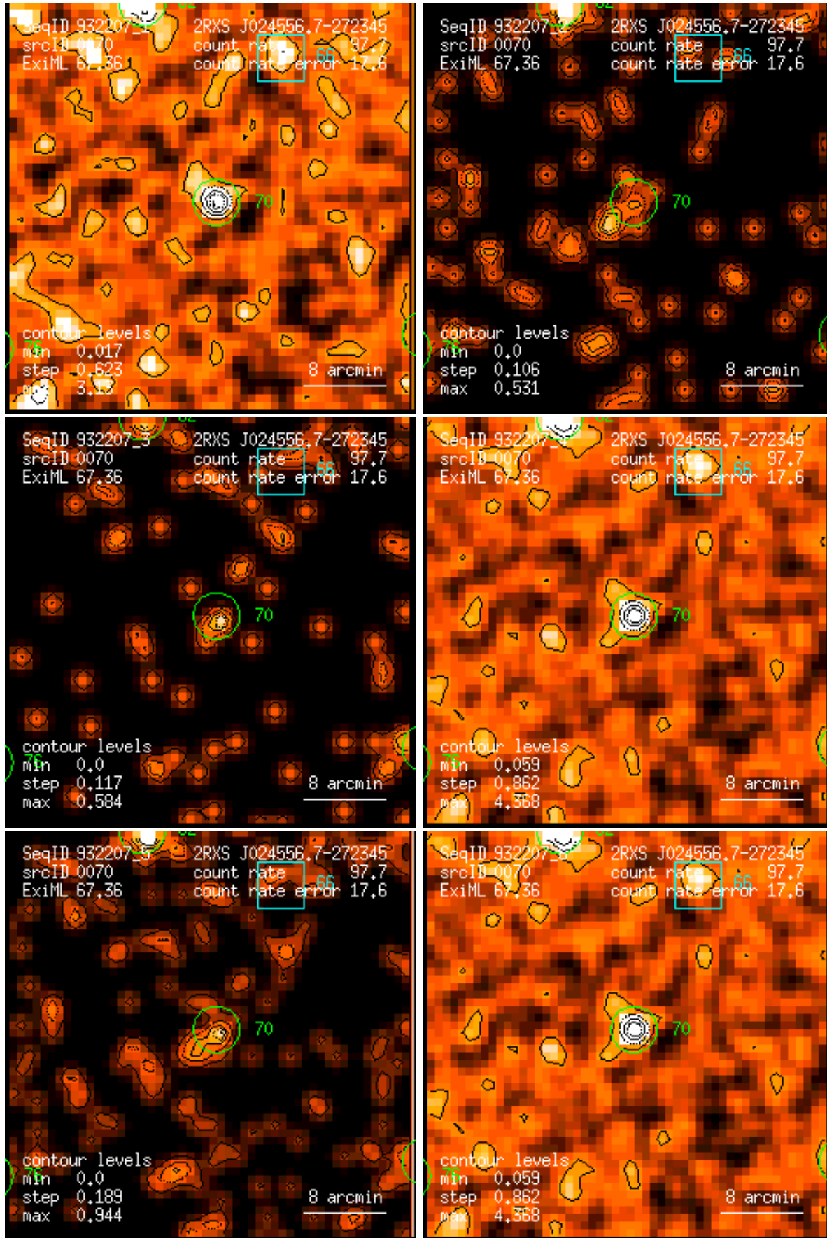
Figure 70: RASS 932207: detection 0070: band rate images, Gaussian filter: (1) PSPC channels 11 – 41, (2) 52 – 90, (3) 91 – 201, (4) 11 – 235, (5) 52 – 201, (6) 11 – 201. Broad band rates in counts/ks. Band rate contour levels in counts/ks/arcmin 2 .
