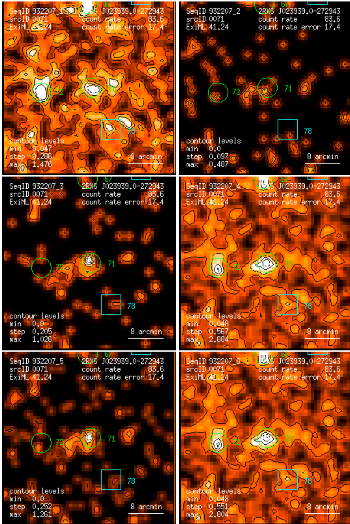
Figure 71: RASS 932207: detection 0071: band rate images, Gaussian filter: (1) PSPC channels 11 – 41, (2) 52 – 90, (3) 91 – 201, (4) 11 – 235, (5) 52 – 201, (6) 11 – 201. Broad band rates in counts/ks. Band rate contour levels in counts/ks/arcmin 2 .
