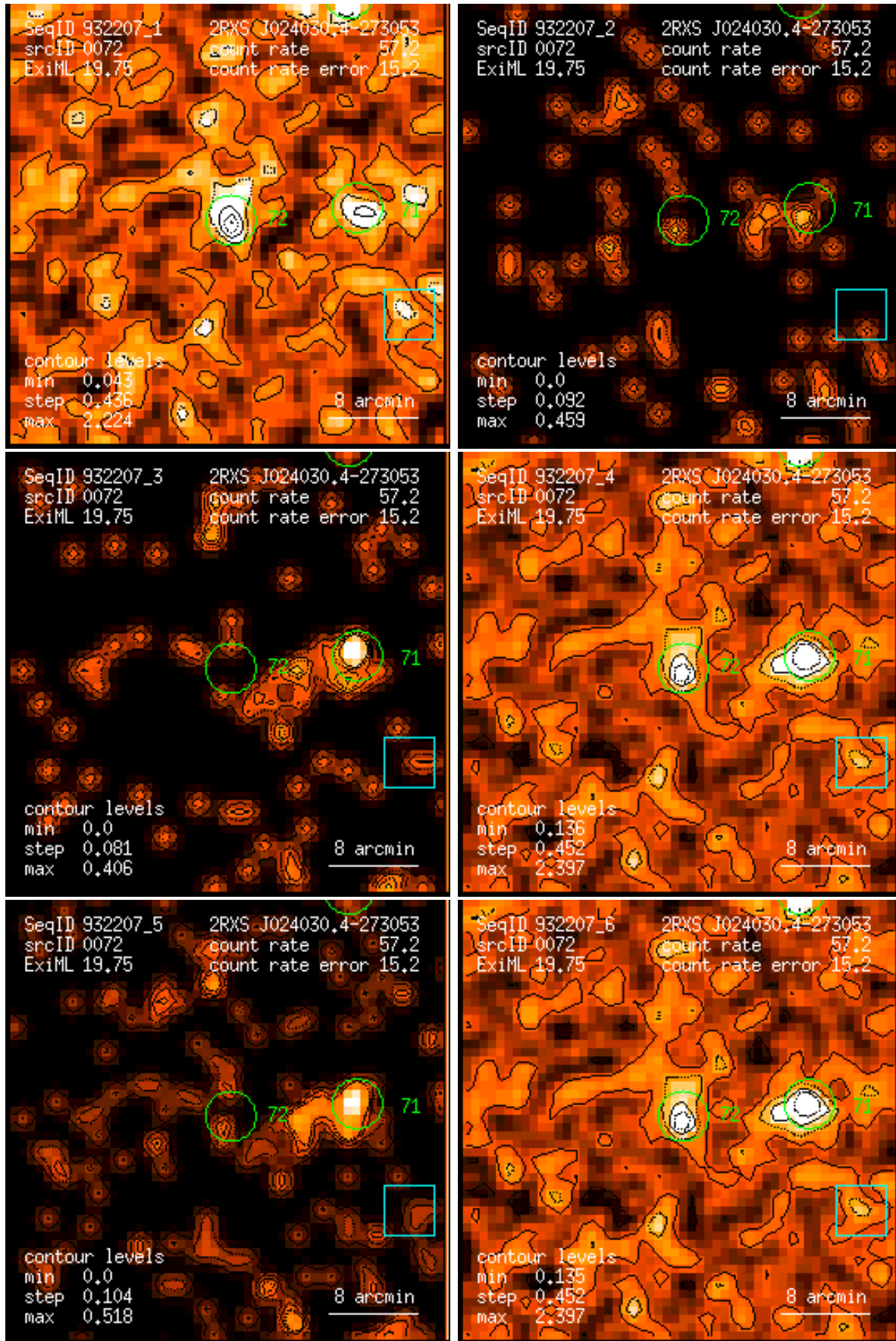
Figure 72: RASS 932207: detection 0072: band rate images, Gaussian filter: (1) PSPC channels 11 – 41, (2) 52 – 90, (3) 91 – 201, (4) 11 – 235, (5) 52 – 201, (6) 11 – 201. Broad band rates in counts/ks. Band rate contour levels in counts/ks/arcmin 2 .
