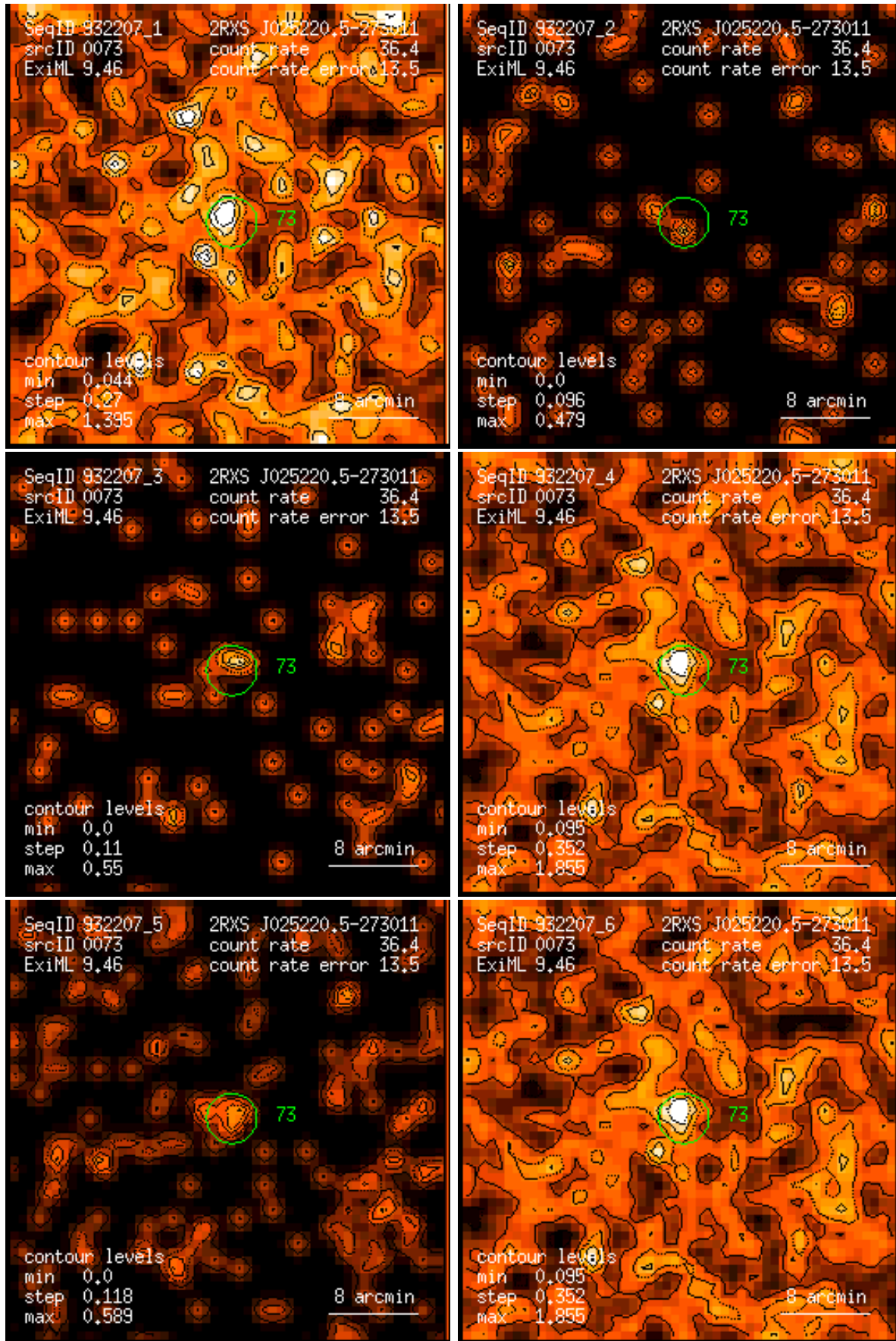
Figure 73: RASS 932207: detection 0073: band rate images, Gaussian filter: (1) PSPC channels 11 – 41, (2) 52 – 90, (3) 91 – 201, (4) 11 – 235, (5) 52 – 201, (6) 11 – 201. Broad band rates in counts/ks. Band rate contour levels in counts/ks/arcmin 2 .
