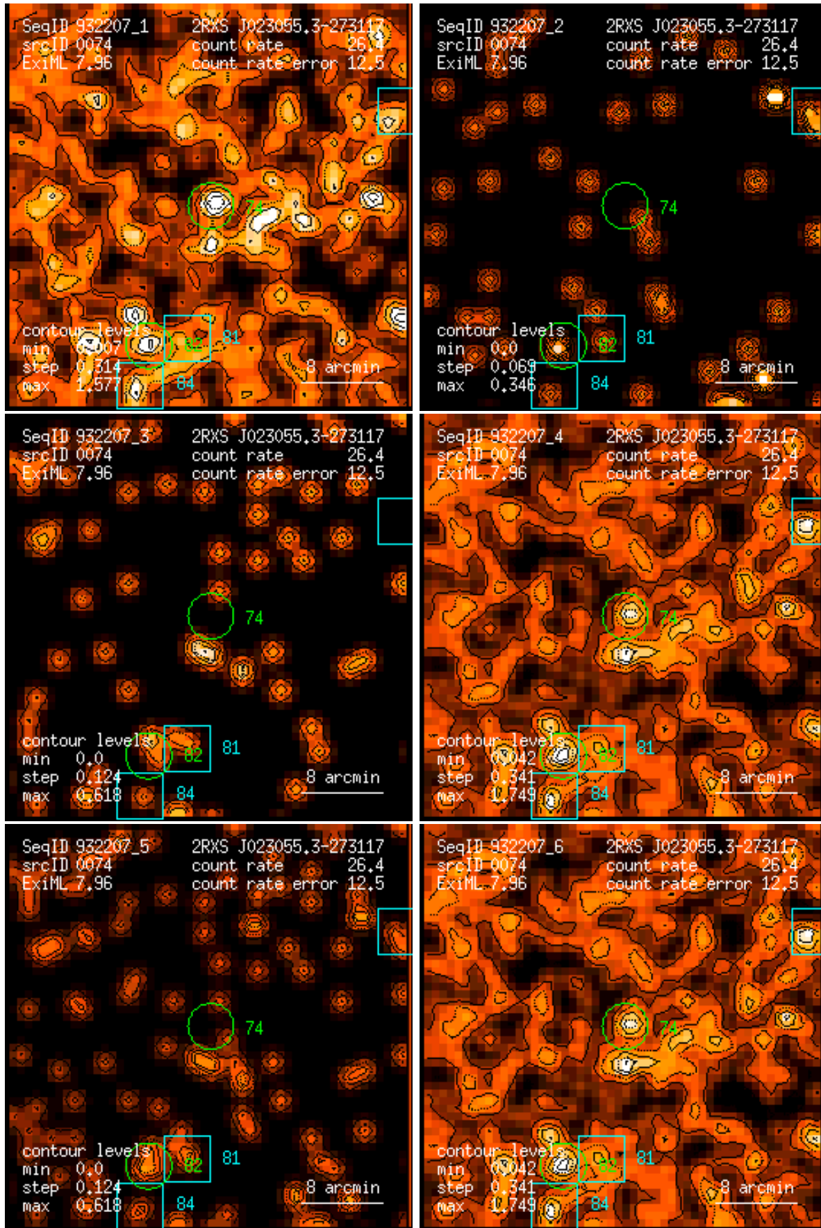
Figure 74: RASS 932207: detection 0074: band rate images, Gaussian filter: (1) PSPC channels 11 – 41, (2) 52 – 90, (3) 91 – 201, (4) 11 – 235, (5) 52 – 201, (6) 11 – 201. Broad band rates in counts/ks. Band rate contour levels in counts/ks/arcmin 2 .
