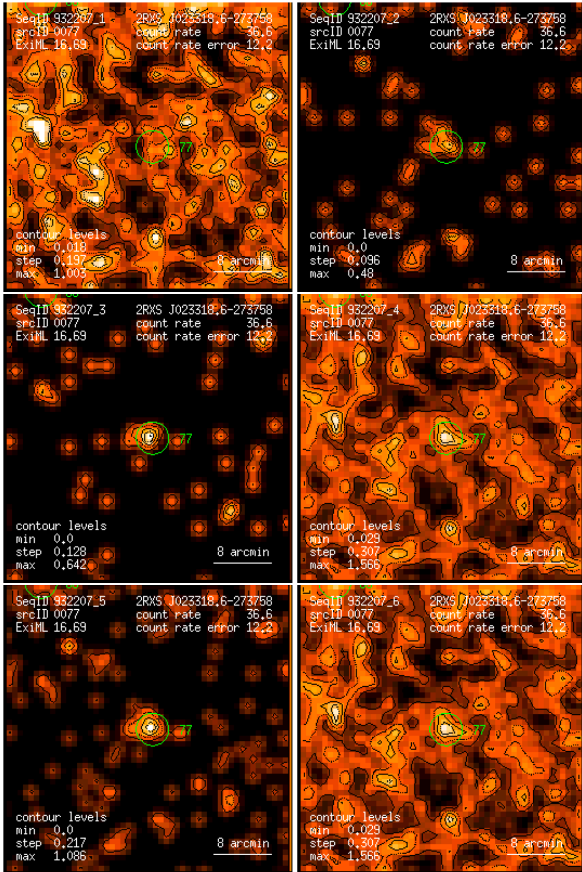
Figure 77: RASS 932207: detection 0077: band rate images, Gaussian filter: (1) PSPC channels 11 – 41, (2) 52 – 90, (3) 91 – 201, (4) 11 – 235, (5) 52 – 201, (6) 11 – 201. Broad band rates in counts/ks. Band rate contour levels in counts/ks/arcmin 2 .
