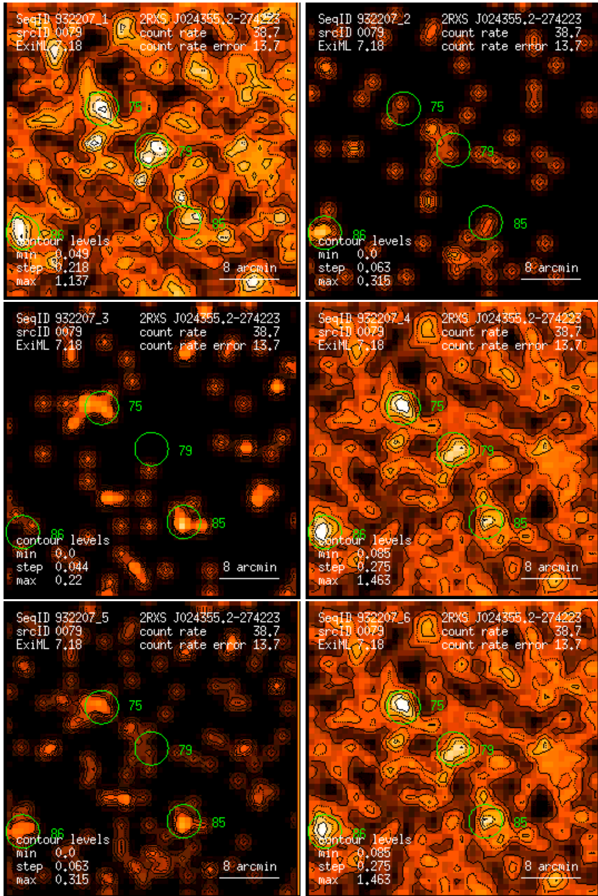
Figure 79: RASS 932207: detection 0079: band rate images, Gaussian filter: (1) PSPC channels 11 – 41, (2) 52 – 90, (3) 91 – 201, (4) 11 – 235, (5) 52 – 201, (6) 11 – 201. Broad band rates in counts/ks. Band rate contour levels in counts/ks/arcmin 2 .
