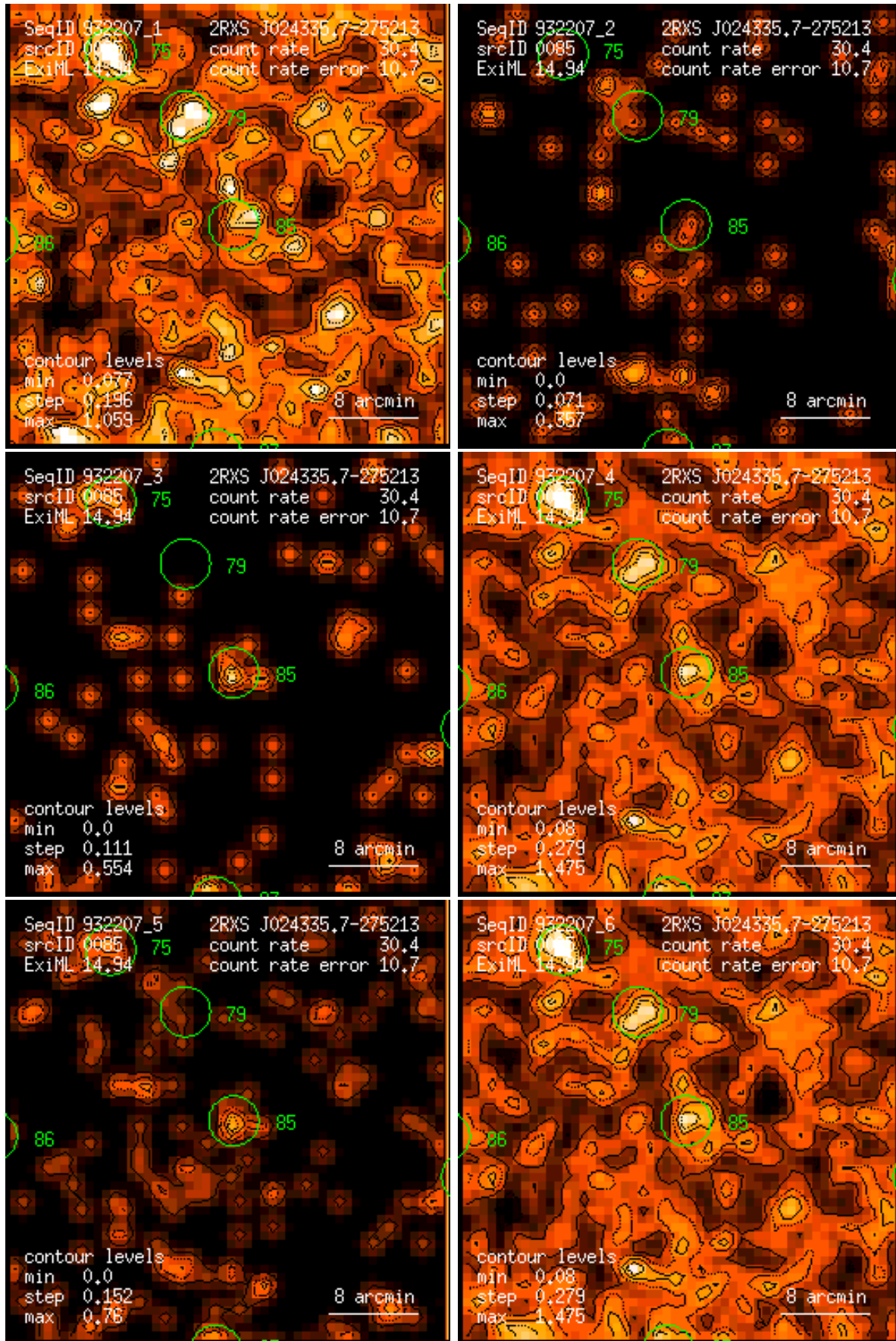
Figure 85: RASS 932207: detection 0085: band rate images, Gaussian filter: (1) PSPC channels 11 – 41, (2) 52 – 90, (3) 91 – 201, (4) 11 – 235, (5) 52 – 201, (6) 11 – 201. Broad band rates in counts/ks. Band rate contour levels in counts/ks/arcmin 2 .
