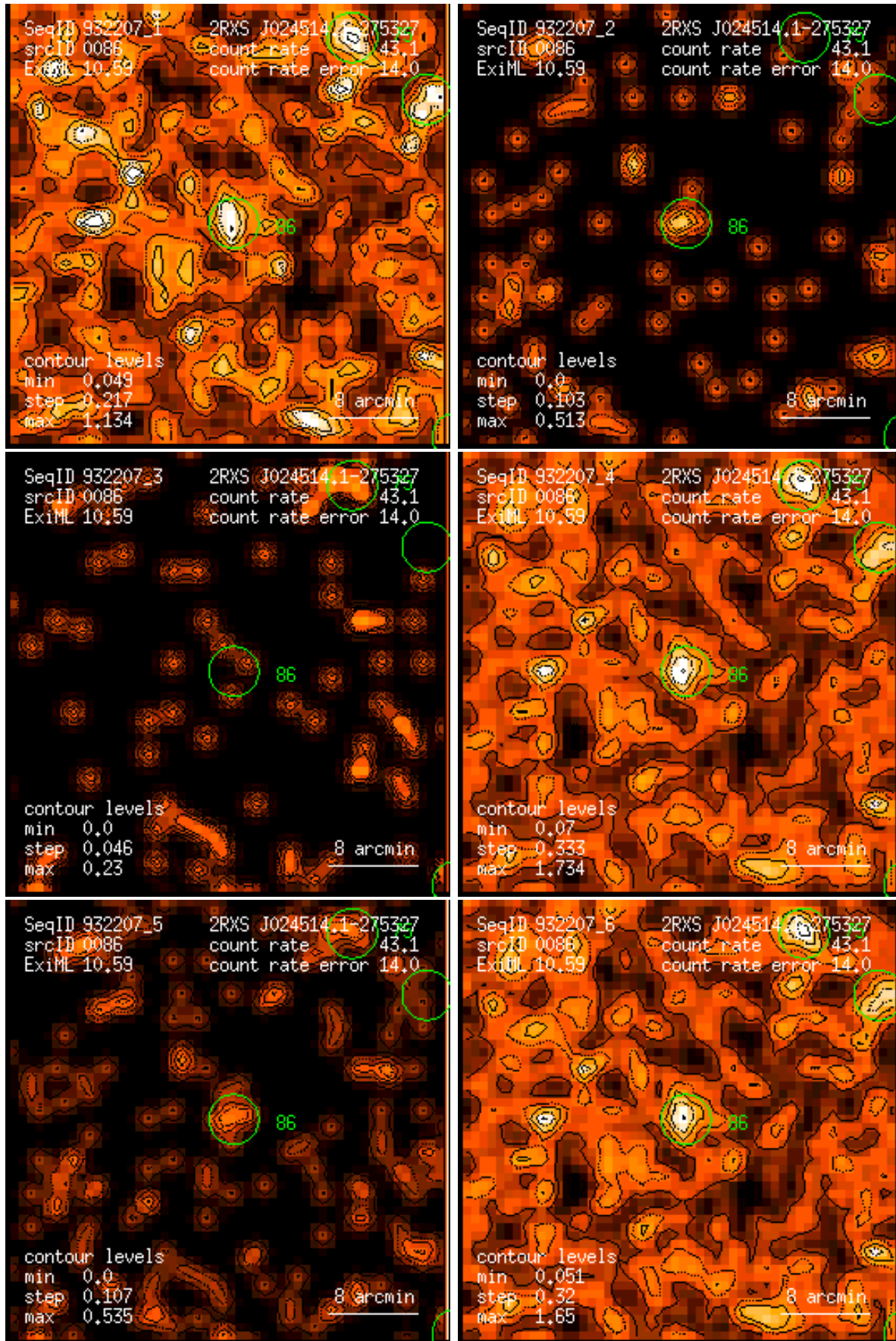
Figure 86: RASS 932207: detection 0086: band rate images, Gaussian filter: (1) PSPC channels 11 – 41, (2) 52 – 90, (3) 91 – 201, (4) 11 – 235, (5) 52 – 201, (6) 11 – 201. Broad band rates in counts/ks. Band rate contour levels in counts/ks/arcmin 2 .
