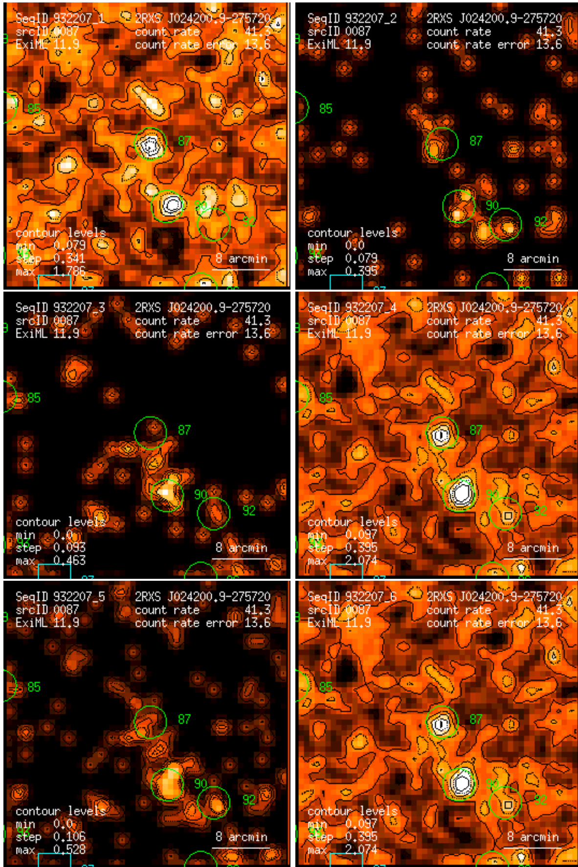
Figure 87: RASS 932207: detection 0087: band rate images, Gaussian filter: (1) PSPC channels 11 – 41, (2) 52 – 90, (3) 91 – 201, (4) 11 – 235, (5) 52 – 201, (6) 11 – 201. Broad band rates in counts/ks. Band rate contour levels in counts/ks/arcmin 2 .
