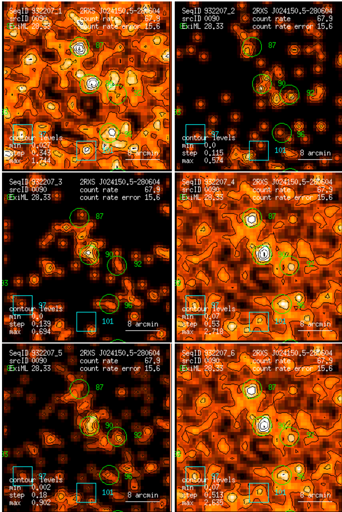
Figure 90: RASS 932207: detection 0090: band rate images, Gaussian filter: (1) PSPC channels 11 – 41, (2) 52 – 90, (3) 91 – 201, (4) 11 – 235, (5) 52 – 201, (6) 11 – 201. Broad band rates in counts/ks. Band rate contour levels in counts/ks/arcmin 2 .
