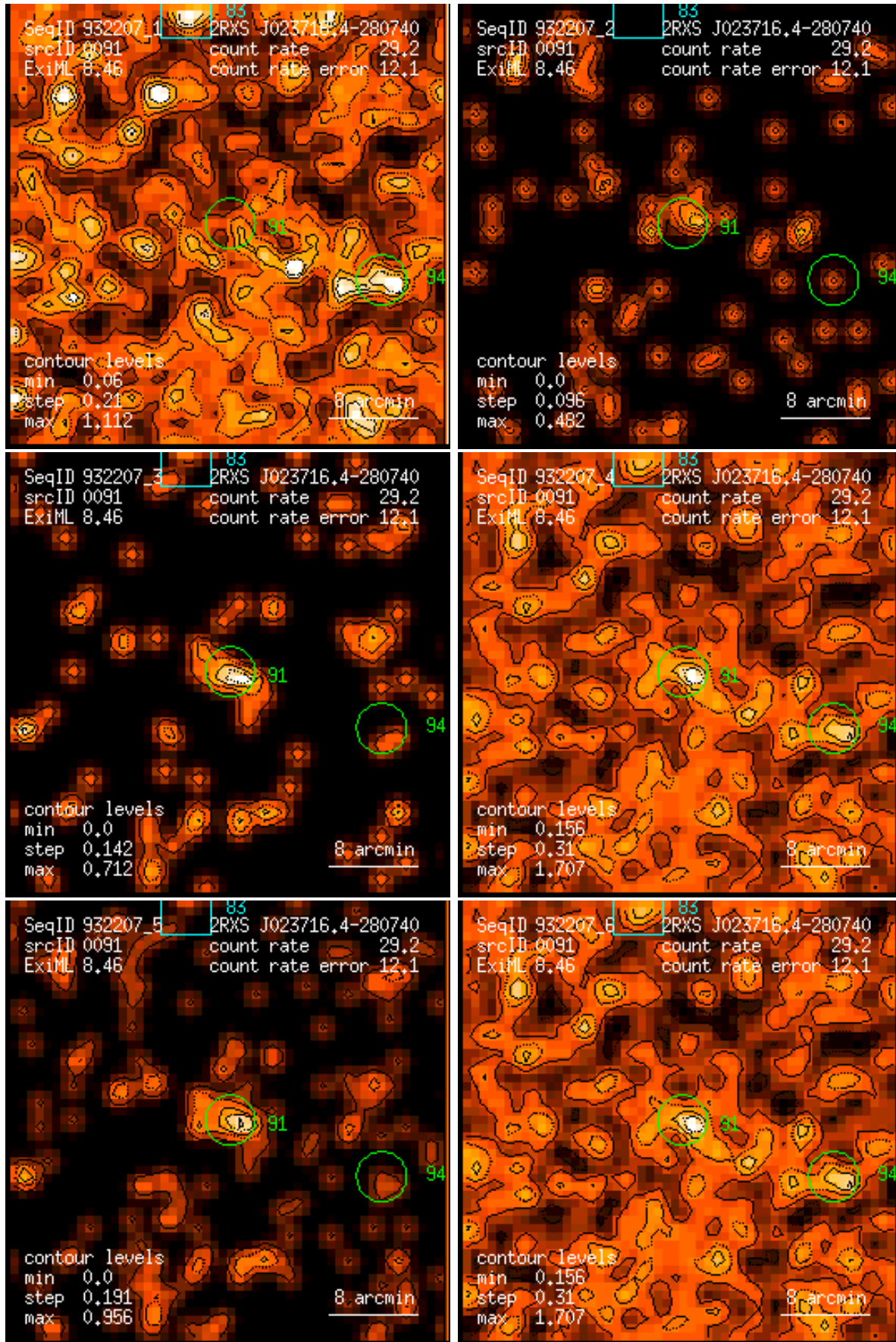
Figure 91: RASS 932207: detection 0091: band rate images, Gaussian filter: (1) PSPC channels 11 – 41, (2) 52 – 90, (3) 91 – 201, (4) 11 – 235, (5) 52 – 201, (6) 11 – 201. Broad band rates in counts/ks. Band rate contour levels in counts/ks/arcmin 2 .
