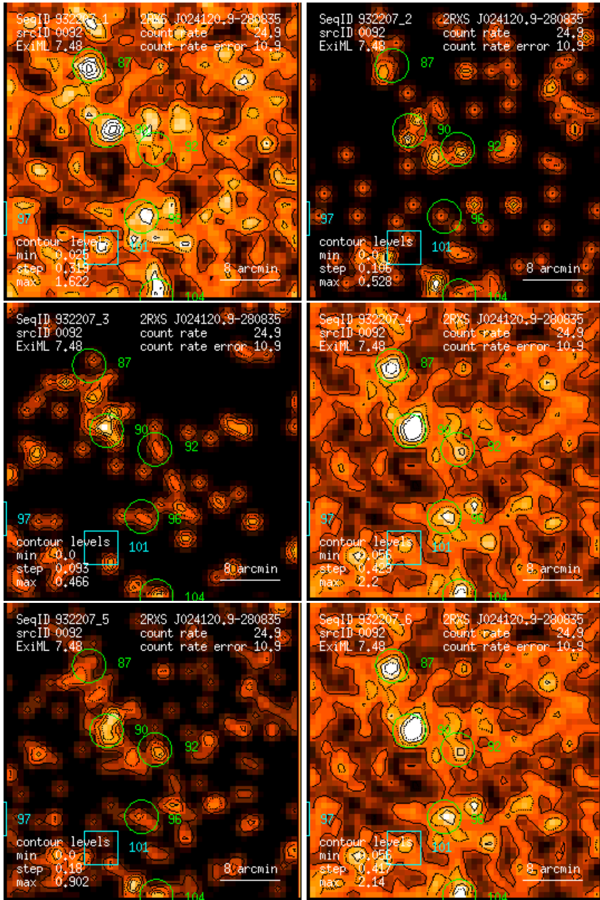
Figure 92: RASS 932207: detection 0092: band rate images, Gaussian filter: (1) PSPC channels 11 – 41, (2) 52 – 90, (3) 91 – 201, (4) 11 – 235, (5) 52 – 201, (6) 11 – 201. Broad band rates in counts/ks. Band rate contour levels in counts/ks/arcmin 2 .
