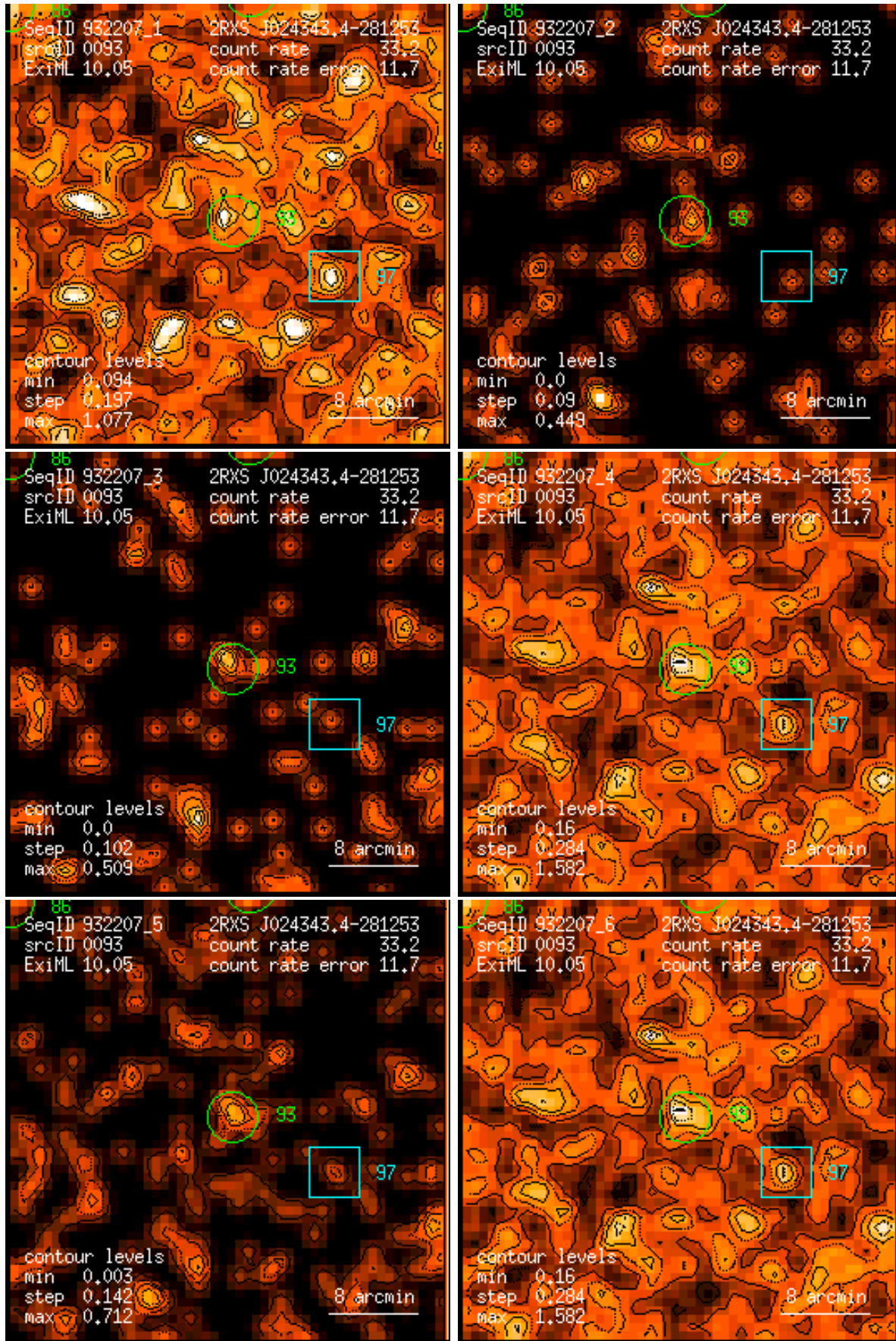
Figure 93: RASS 932207: detection 0093: band rate images, Gaussian filter: (1) PSPC channels 11 – 41, (2) 52 – 90, (3) 91 – 201, (4) 11 – 235, (5) 52 – 201, (6) 11 – 201. Broad band rates in counts/ks. Band rate contour levels in counts/ks/arcmin 2 .
