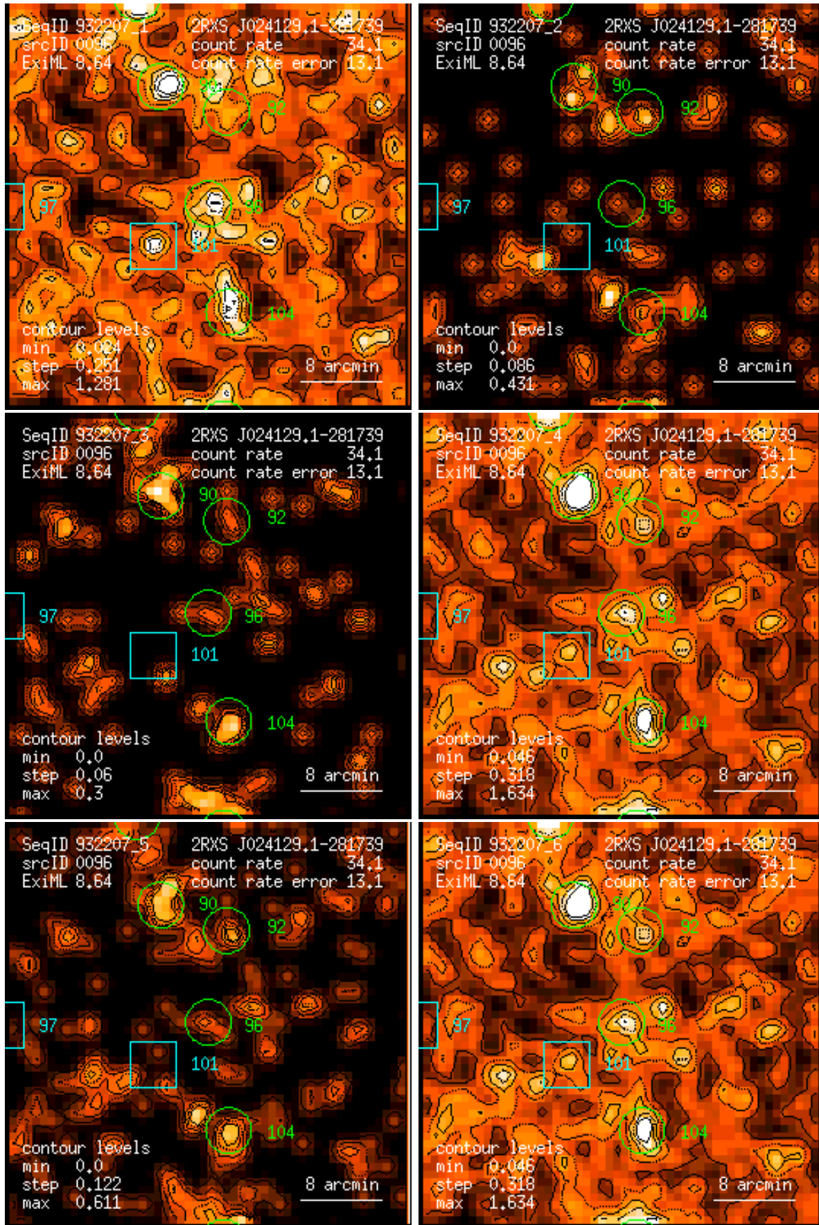
Figure 96: RASS 932207: detection 0096: band rate images, Gaussian filter: (1) PSPC channels 11 – 41, (2) 52 – 90, (3) 91 – 201, (4) 11 – 235, (5) 52 – 201, (6) 11 – 201. Broad band rates in counts/ks. Band rate contour levels in counts/ks/arcmin 2 .
