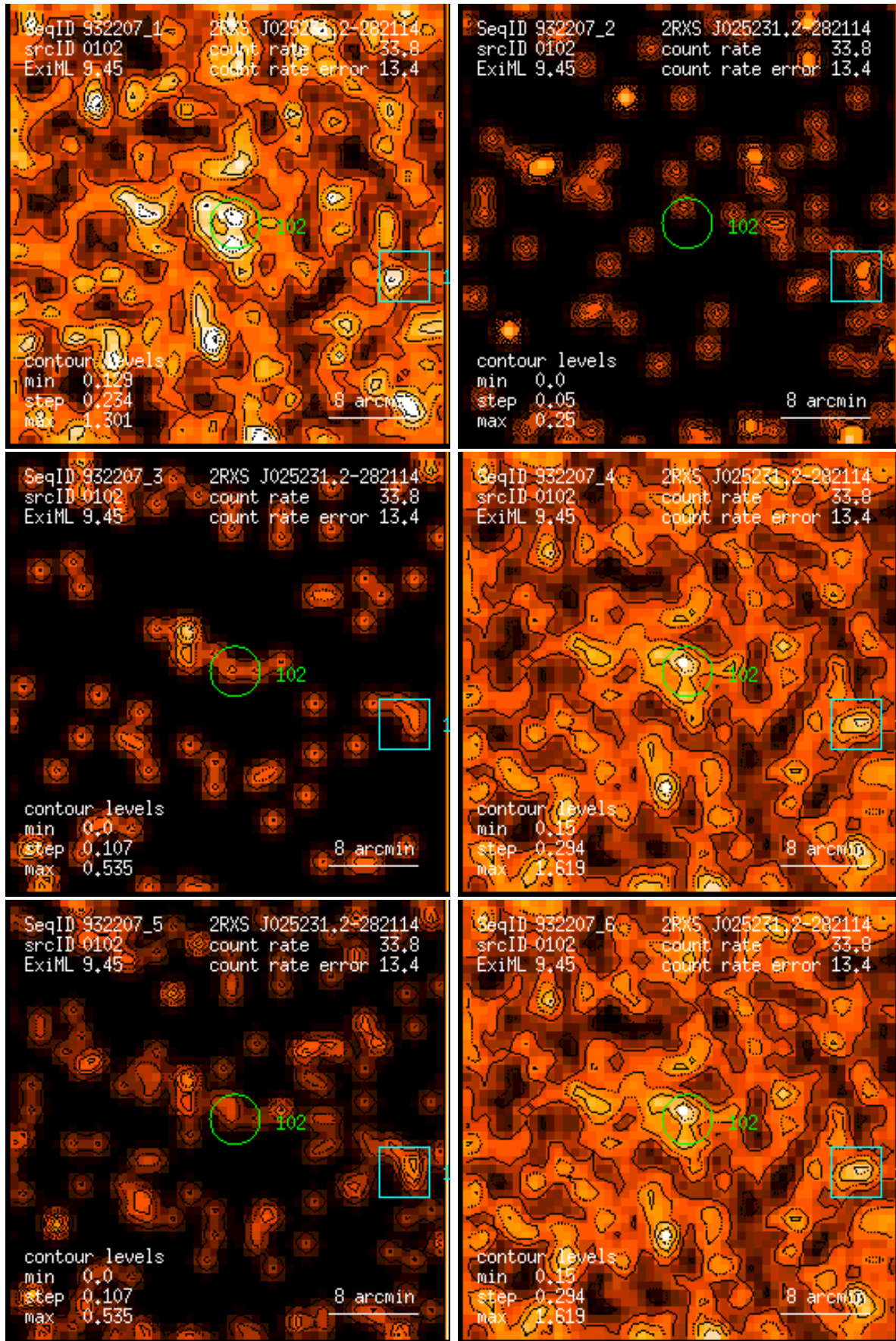
Figure 102: RASS 932207: detection 0102: band rate images, Gaussian filter: (1) PSPC channels 11 – 41, (2) 52 – 90, (3) 91 – 201, (4) 11 – 235, (5) 52 – 201, (6) 11 – 201. Broad band rates in counts/ks. Band rate contour levels in counts/ks/arcmin 2 .
